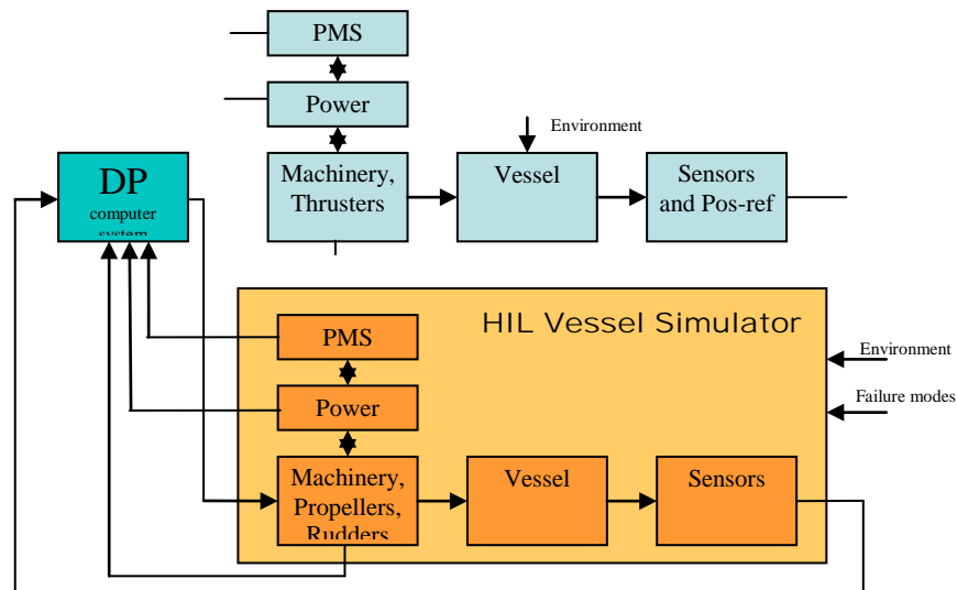
Fig.3. HIL Vessel simulator is typically used at manufacturer works where the simulator represents the vessels systems, the external environment and failure modes are generated and sent to the target DP computer system.
