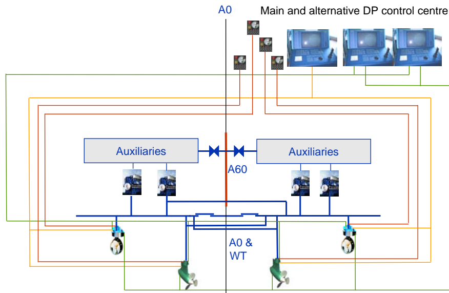
Fig.2. Principle arrangement for DYNPOS-ER notation
