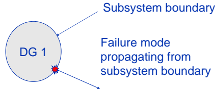
Fig.9. Subsystem boundary for a diesel generator (DG 1). A failure mode is the failure effect observed at the subsystem boundary. For a diesel generator a failure mode is 'Fail to start on demand'
