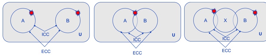
Fig.7. Common cause failure, resulting from a single event related to U, e.g. either as an external (ECC) or an (ICC) internal common cause. (E.g. fire and flooding, environment, vibration, high seas affecting contamination in fuel tanks, shocks, humidity, EMC,....)
