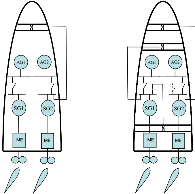
Fig.1. The thruster configuration indicated at the left figure will be acceptable for DPS 0 and DPS 1, but will not be acceptable for DYNPOS-AUTS and DYNPOS-AUT. The thruster configuration indicated at the right figure will be acceptable for DPS 2, but will not be acceptable for DYNPOS-AUTR
