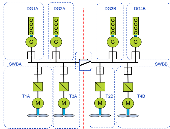
Fig.5. The redundancy design intention in this example may be described in an e.g. narrative way by describing both the normal operation mode and the failed operation mode.
