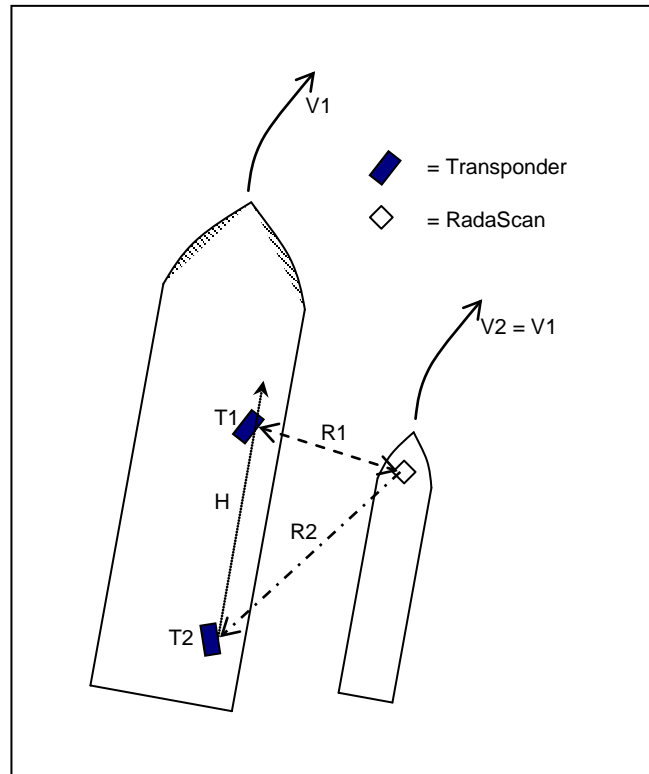
Figure 5: RAS vessel configuration
