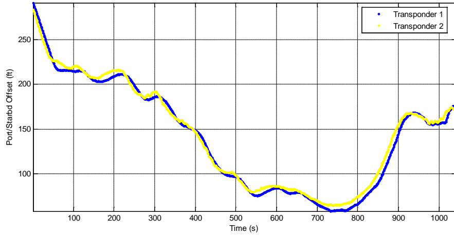
Figure 6(a): RadaScan transponder port / starboard offset during a RAS maneuver
