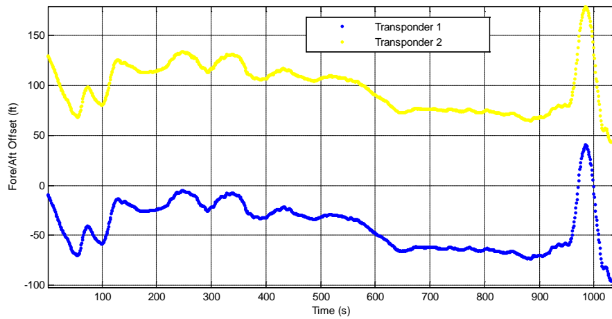
Figure 6(b): RadaScan transponder fore/aft data during a RAS maneuver
