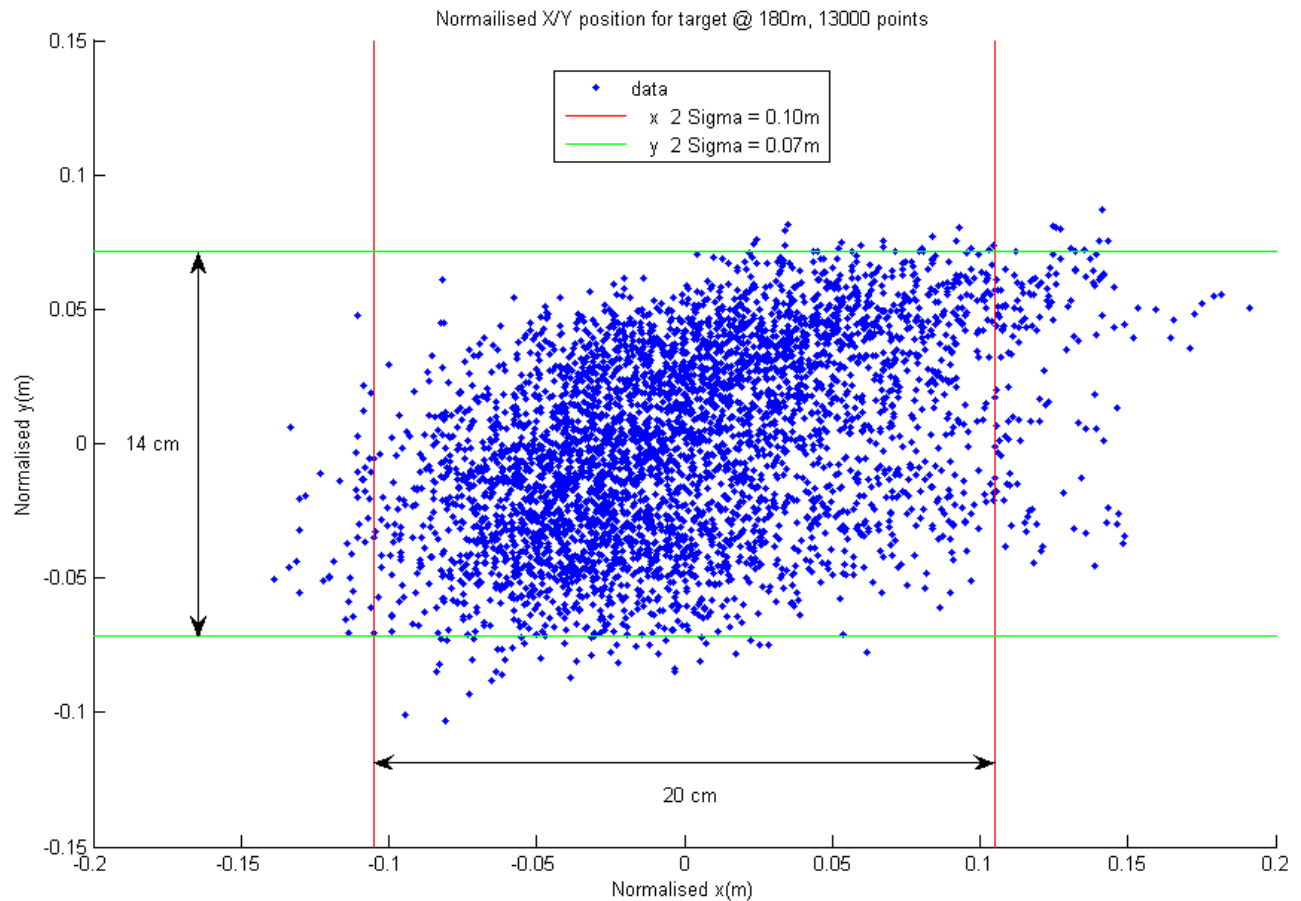
Figure 4: RadaScan transponder position plot at 180m (590feet)
