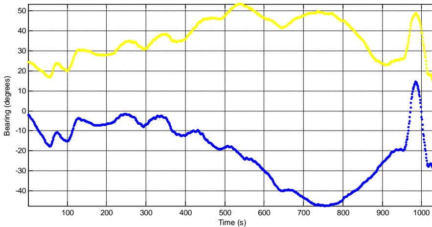
Figure 6(c): RadaScan transponder bearing data during a RAS maneuver
