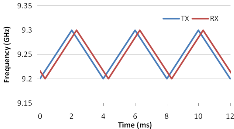
Figure 2: RadaScan FMCW Radar Output and Return Signals
