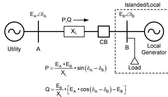
Fig. 3 Simplified Utility Power System
