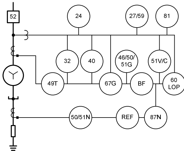
Fig. 7 Standard Features of Generator Protection Relay
