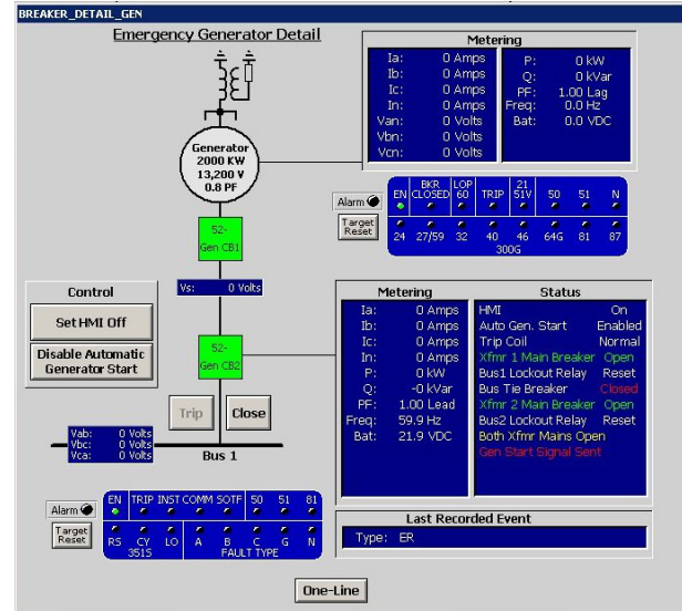
Fig. 10 Example Black-Start Generation Fault
