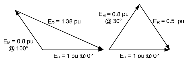
Fig. 6 High-Speed Motor Transfer (Resultant Voltage)
