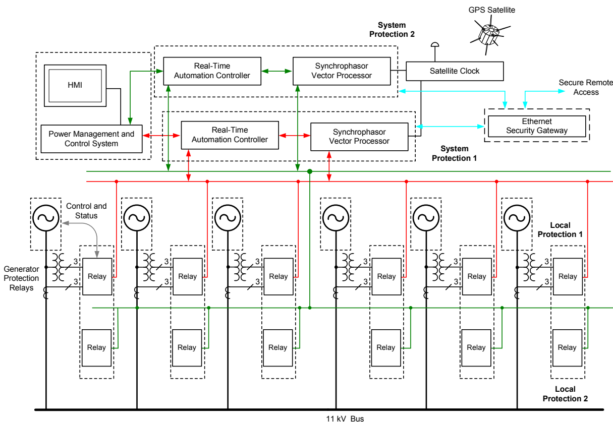
Fig. 5 Proposed Solution—Redundant Protection
