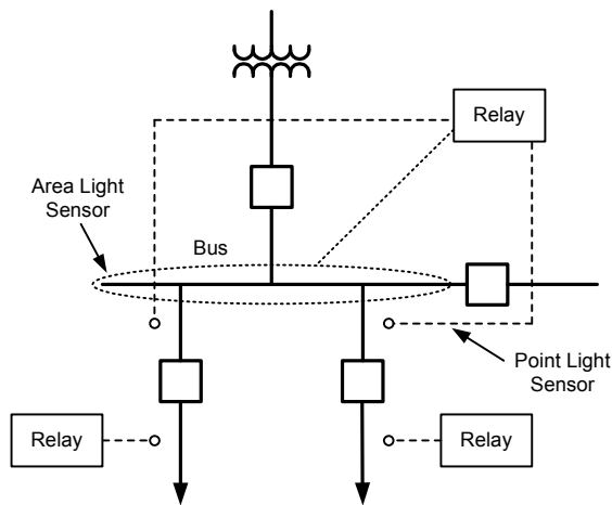
Fig. 13 High-Speed Arc-Flash Detection
