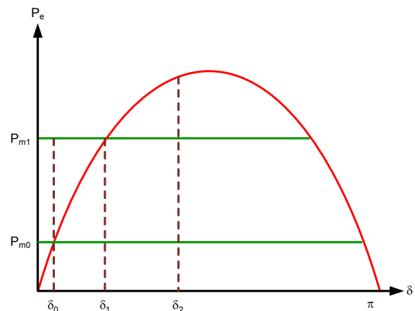
Fig. 4 Power Flow Example
