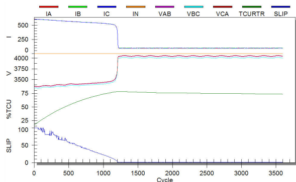
Fig. 15 Example Motor Starting Report
