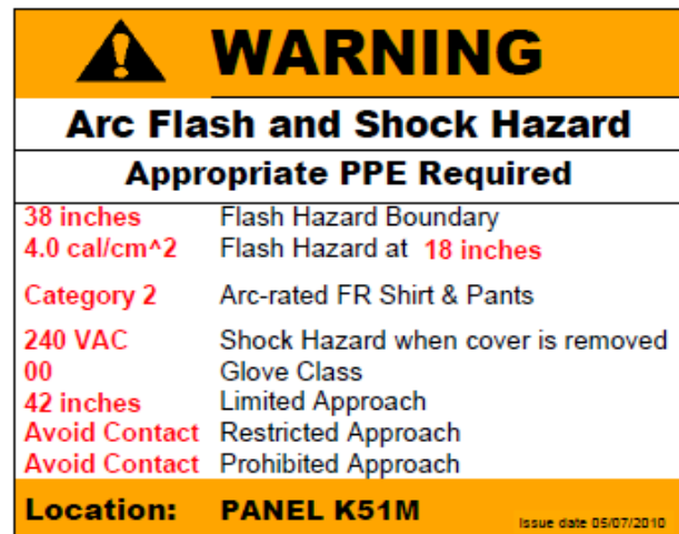
Fig. 14 Example Arc-Flash Label
