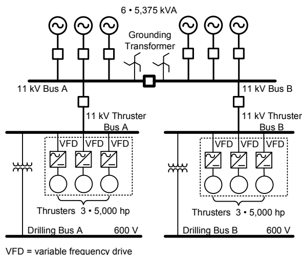
Fig. 1 Simplified Electrical System Example 1
