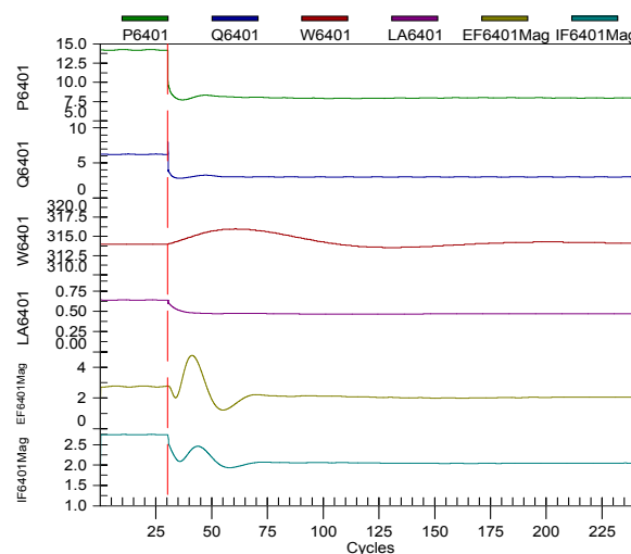
Fig. 16 Generator Results Benchmark Using RTDS
