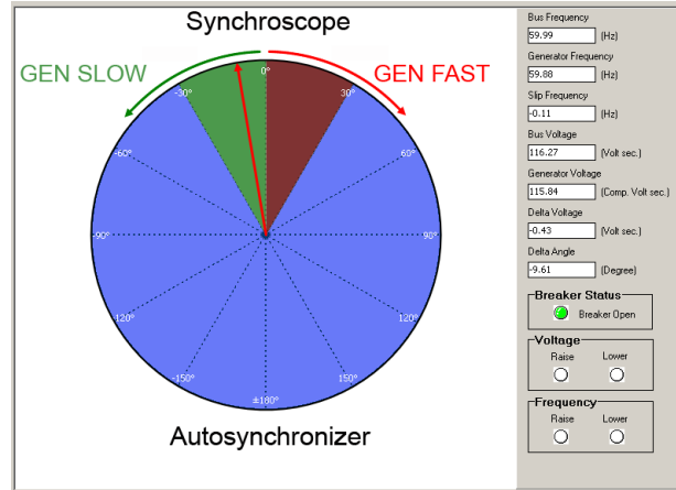
Fig. 8 Automatic Synchronization
