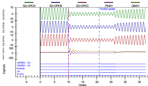
Fig. 11 Example Fault Analysis for the Three-Phase Fault
