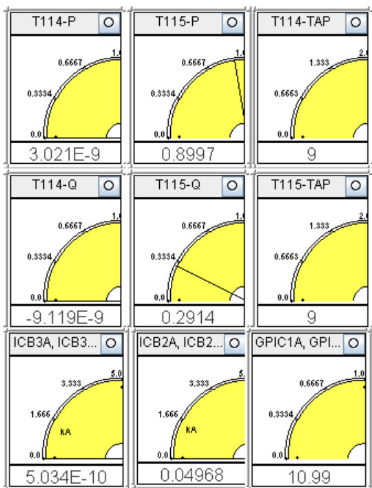
Fig. 17 Example System Results Using RTDS
