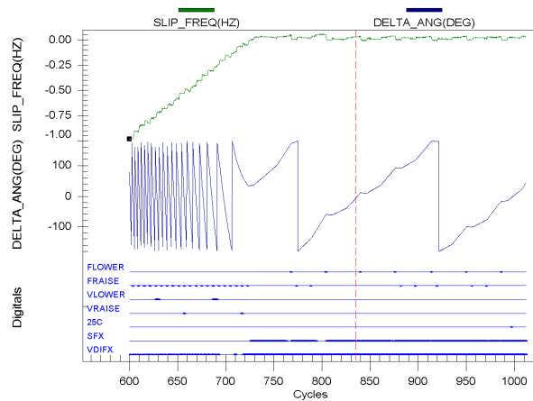
Fig. 9 Example Automatic Synchronization Report
