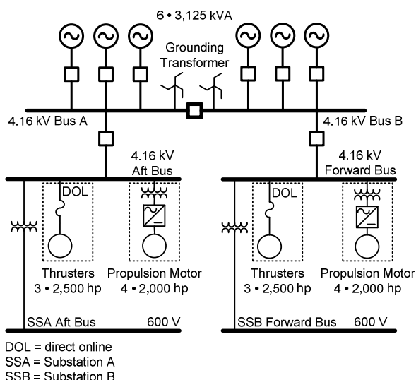
Fig. 2 Simplified Electrical System Example 2
