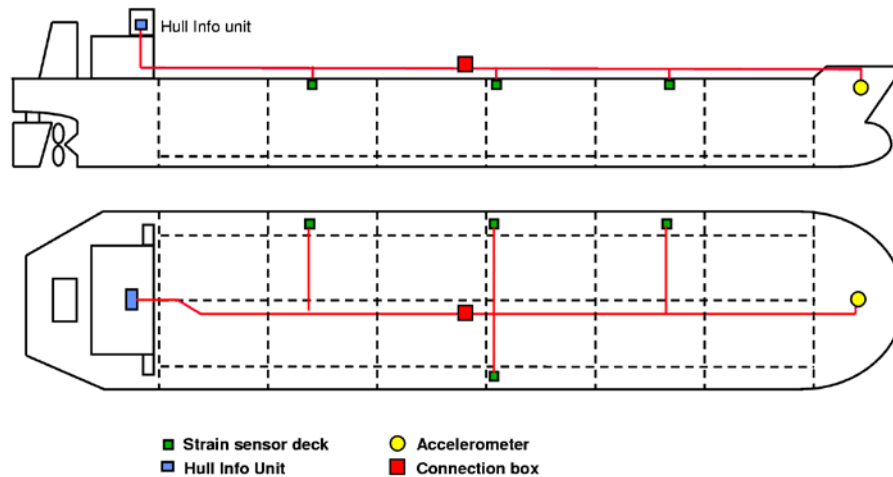
Figure 1: Typical arrangement for measurement of vertical bending moments
