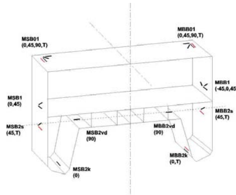
Figure 3: Mid section instrumented with 17 strain sensors to measure 6 global loads
