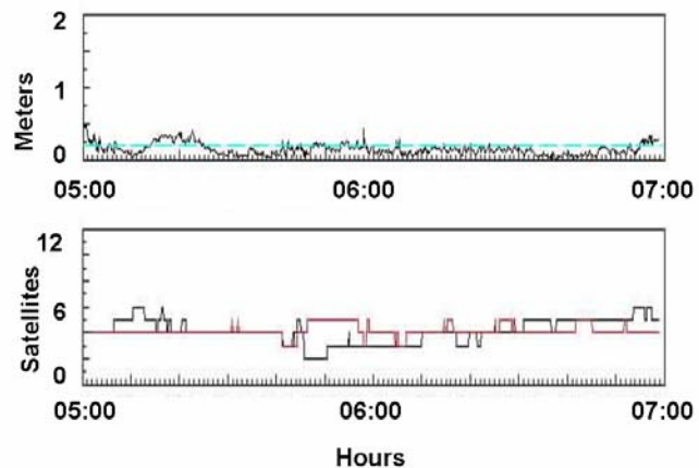
Figure 5: Errors during a two hours test next to an obstruction. The top plot shows horizontal position error and the bottom plot shows the number GPS (black) and GLONASS (red) satellites,
