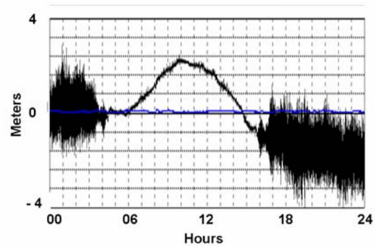
Figure 9: Relative height during 24 hours on Bourbon Topaz 16 October 2008. The vessel is at harbor between 0400 and 1600 where the tidal variation can be seen.
