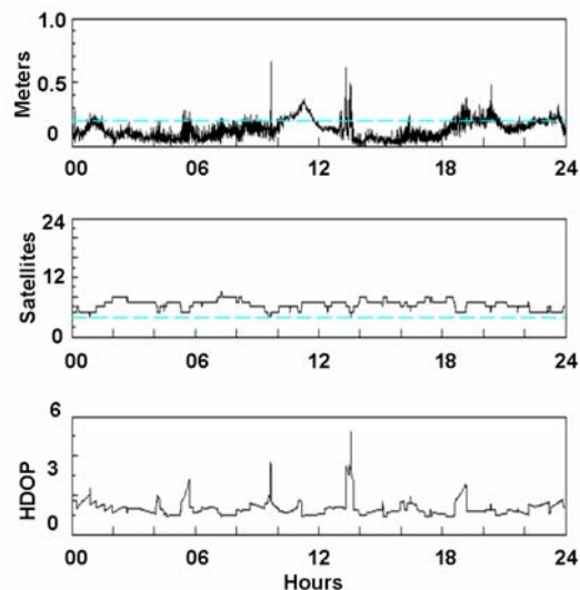
Figure 10: Static performance using GLONASS-only data on 28 March 2009. The top plot is horizontal position error, the middle plot the number of satellites used in the solution and the bottom plot HDOP.
