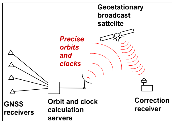
Figure 1: G2 data flow overview
