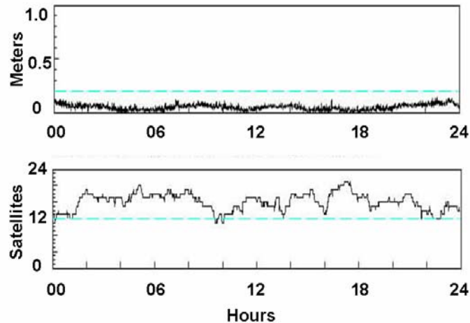
Figure 3: Position performance using GPS and GLONASS on 28 March 2009. The top plot is horizontal position error, and the bottom plot the number of satellites used in the solution.
