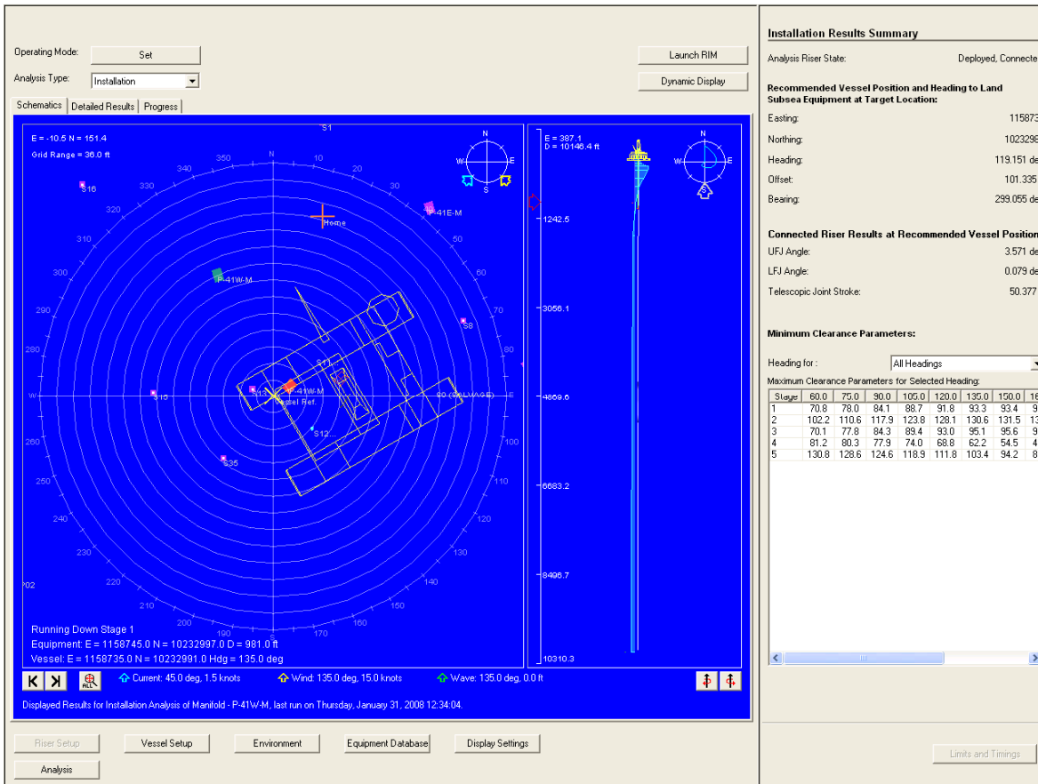
Figure 2. Example of onboard software operator interface
