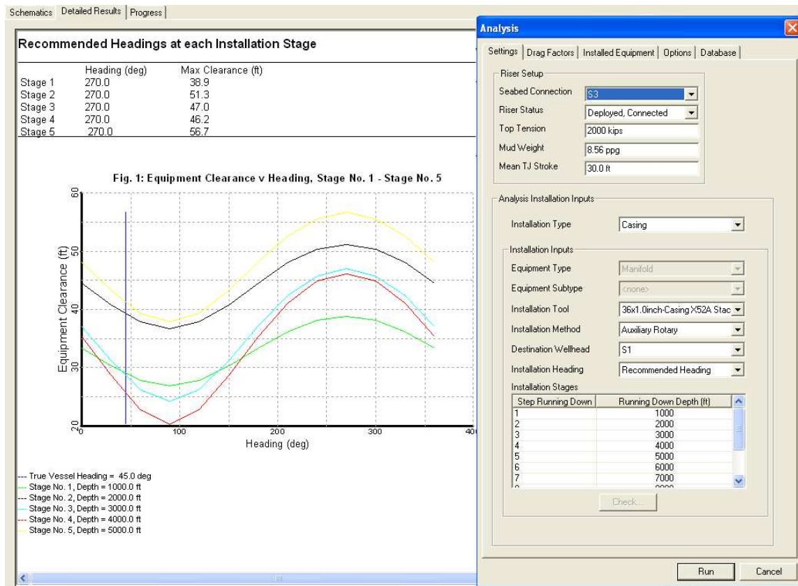
Figure 4. Selected results from casing running example showing how the minimum clearance between the casing and the riser varies with vessel heading. The Analysis Setup dialog is shown on the right.
