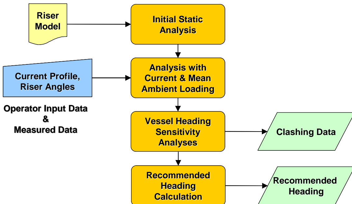
Figure 3. Flowchart for typical SIMOPS simulation
