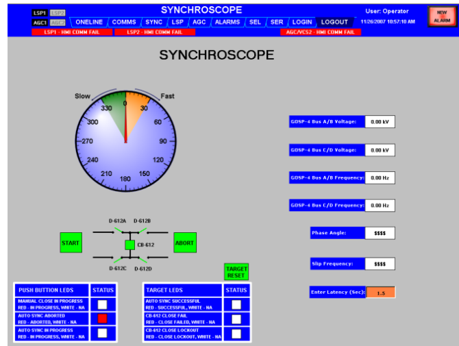
Fig. 8. Automatic Synchronizer
