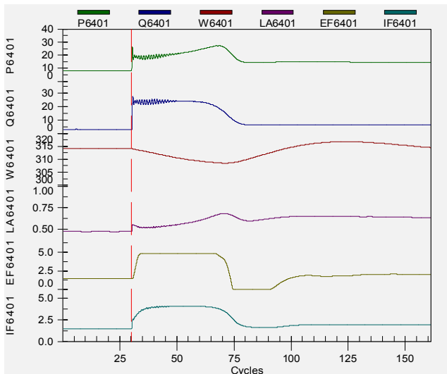
Fig. 17. Results of Step-Load Test Using an RTDS Modeling an Example System
