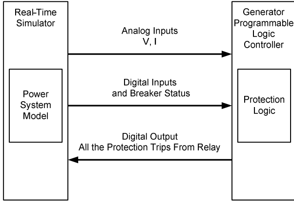
Fig. 16. RTDS and Test Model Connection
