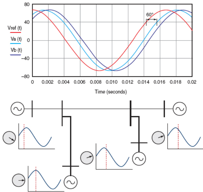
Fig. 6. Synchrophasor Measurement
