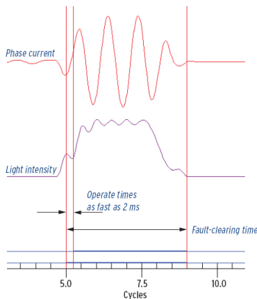
Fig. 10. Arc-Flash Operation Times
