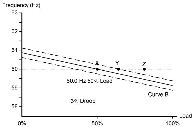
Fig. 12. High kW and Droop Mode
