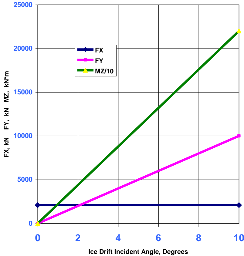
Level ICE t = 2.0 m AARC Report A-392
