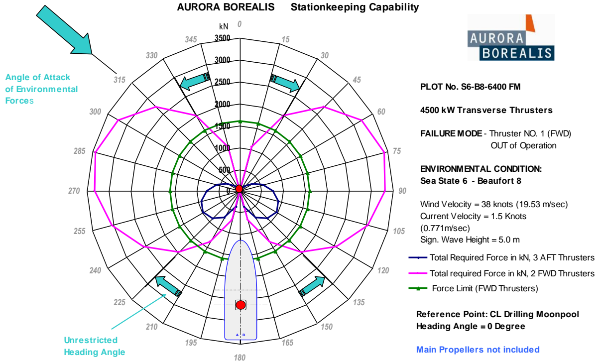
Sample Polar Plot for Stationkeeping in Open Water 4500 kW Thruster, Failure Mode
