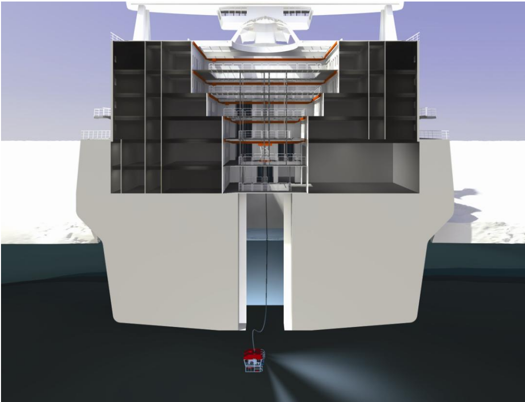
AB section at scientific moon pool, showing the shape of the hull designed for icebreaking in transverse direction.
