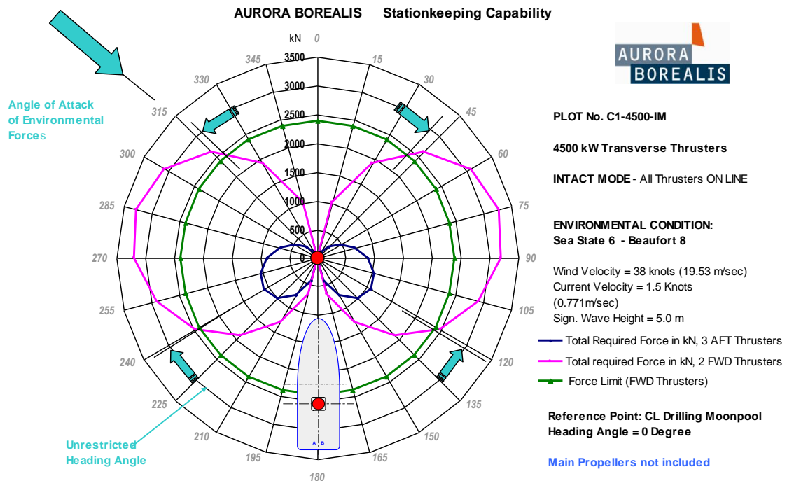
Sample Polar Plot for Stationkeeping in Open Water 4500 kW Thruster, Intact Mode
