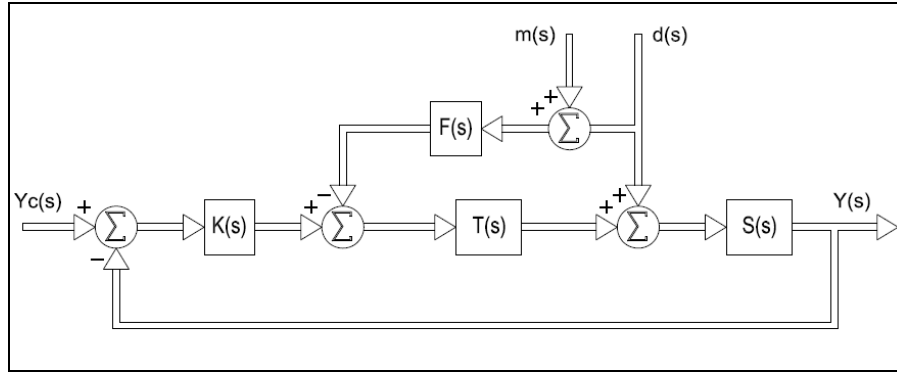
Figure 2: Basic DP system block diagram
