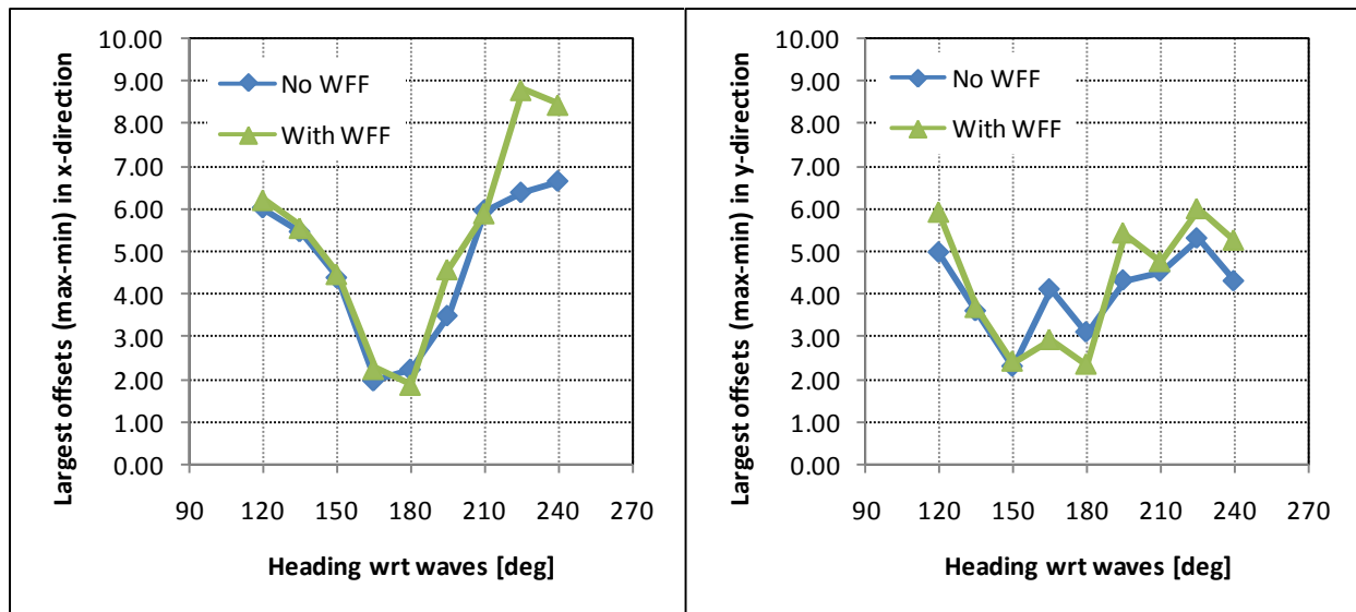
Figure 10: Comparison of maximum swept path for two ships in relative DP with and without wave feedforward
