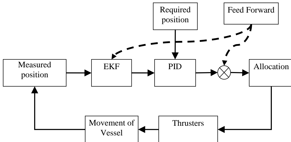
Figure 6: DP control loop with integrated wave feed forward
