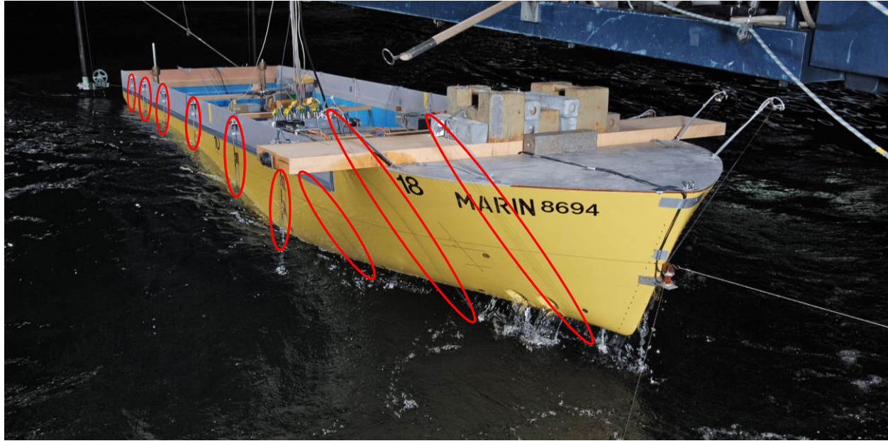
Figure 5: Transshelf equipped with 20 wave probes around the vessel to correlate measured wave forces with local wave height measurements
