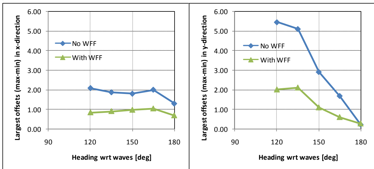
Figure 8: Improvement in watch circle (shown in surge x, and sway y) in sea state 4, for various wave directions, zero speed
