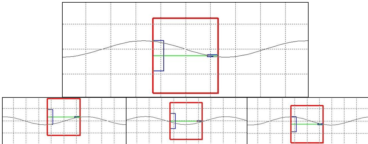
Figure 3: Difference in Wave/Hull Contact Line Near Heave Resonance
