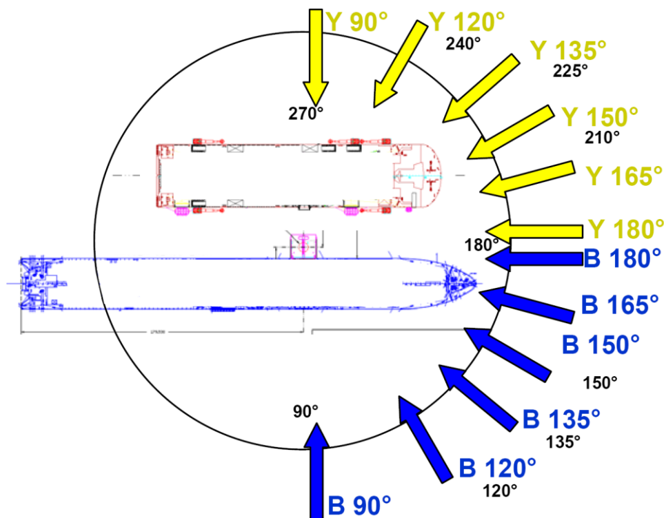
Figure 1: Definition of wave directions with Mighty Servant 3 on lee and on weather side
