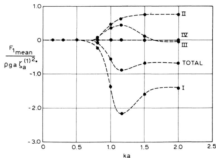
Figure 4: Second Order Wave Load Components
