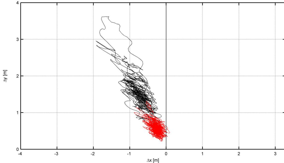
Figure 7: Footprint of trajectory of the centre of gravity, in surge and sway, of the Mighty Servant 3 in Sea State 4, bow quartering waves; WFF disabled (black line) and WFF enabled (red line)
