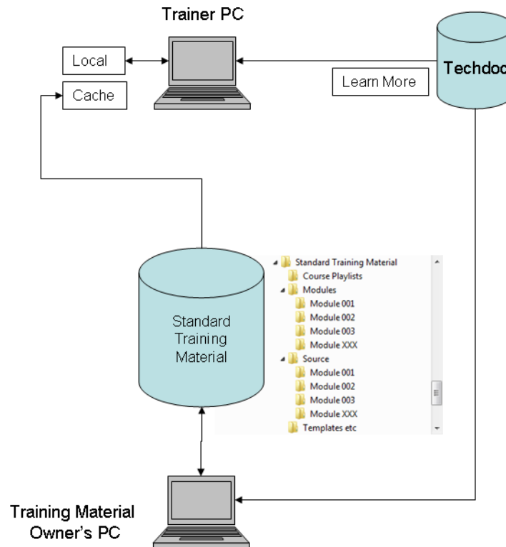
Figure 5 Storage of information used in Nemo™.
