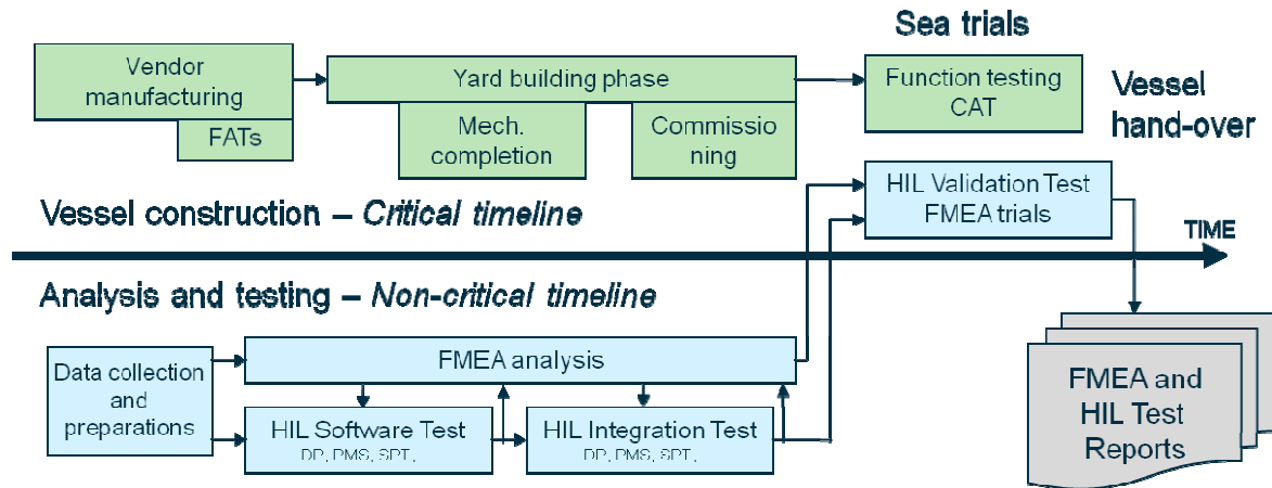
Figure 3: Coordination of HIL and FMEA activities.
