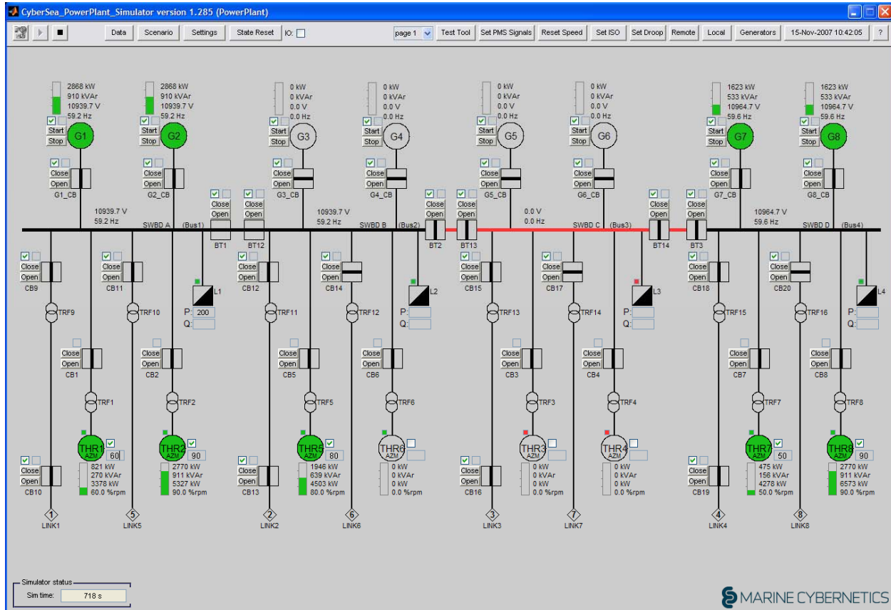
Figure 1: Example of a graphical user interface of a CyberSea Power Plant simulator used to set up scenarios and conduct PMS HIL testing. All key electric parameters such as voltage, frequency, active and reactive power are simulated dynamically in real time at all relevant points of the electric network with resolution of about 100 ms. The dynamic response of electric parameters can be monitored, local control panel functions can be emulated, dynamic loads can be defined and a wide range of failure conditions invoked. The power plant simulator can operate in closed loop taking commands from the PMS and communicating instrument data tags to the PMS.
