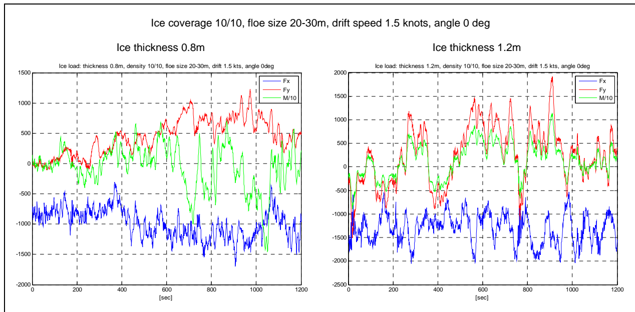
Figure 4 Ice loads at 100% concentration
