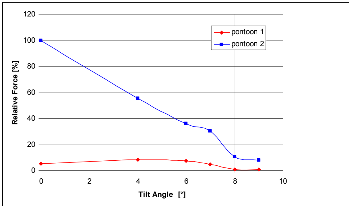
Fig. 11. Transverse forces, acting on both pontoons, the maximum force on pontoon 2 is scaled as 100%.
