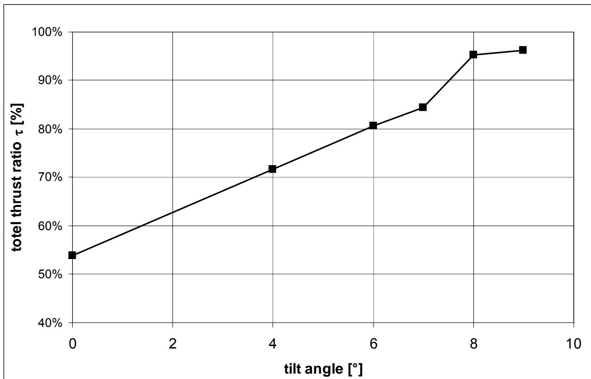
Fig. 6. Total thrust ratio \tau as the function of the tilt angle of the propeller shaft
