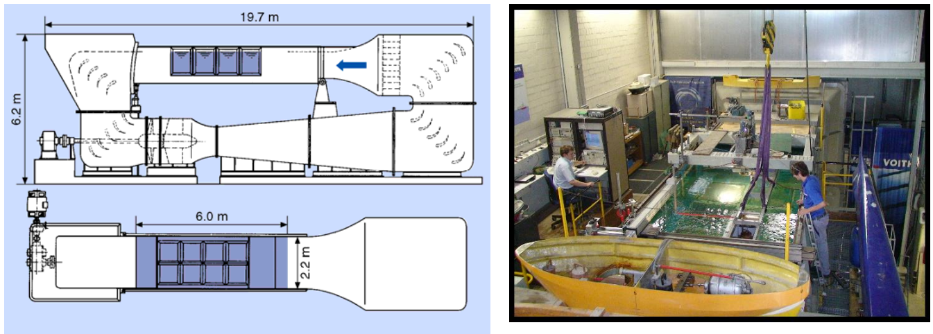
Fig. 12. Tank test facility of Voith Turbo Marine
