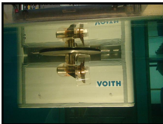
Fig. 13. Measuring arrangement of the 360° steerable thruster
