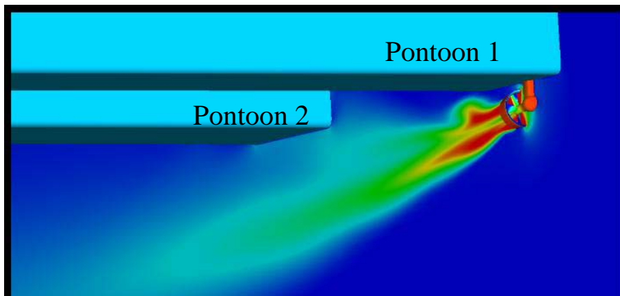
Fig. 4. Arrangement of the pontoons and the thruster with 8° propeller shaft tilting
