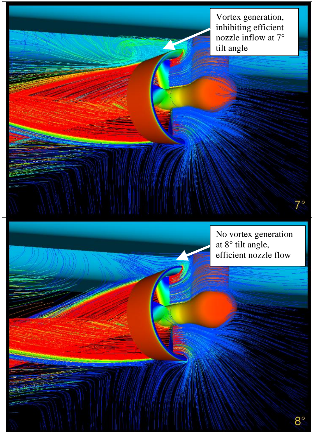
Fig. 7. Flow pattern at 7° and 8° of tilt angle of the propeller shaft
