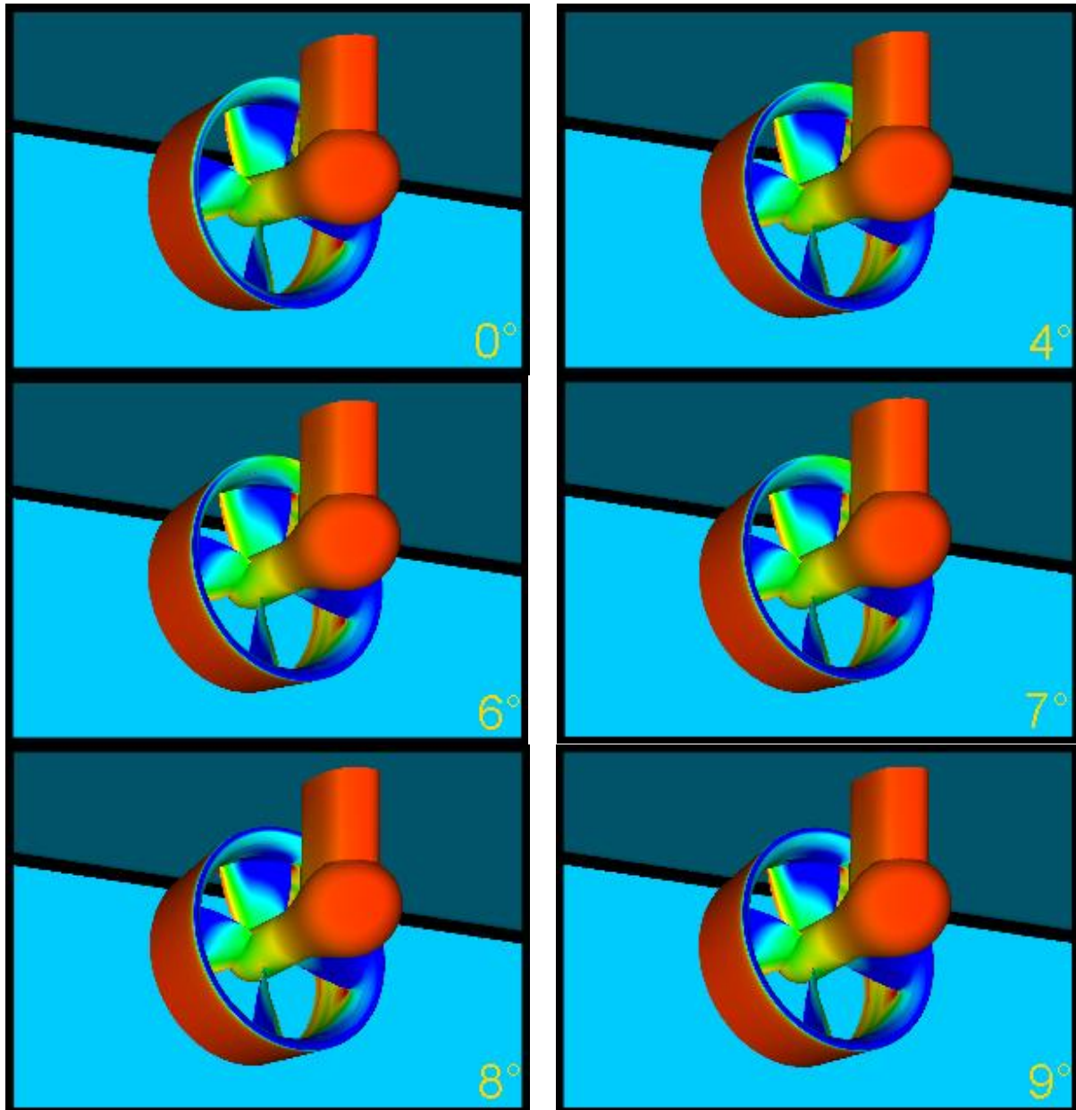
Fig. 10. Pressure Distribution of the azimuthing thruster at different tilt angles of the propeller shaft
