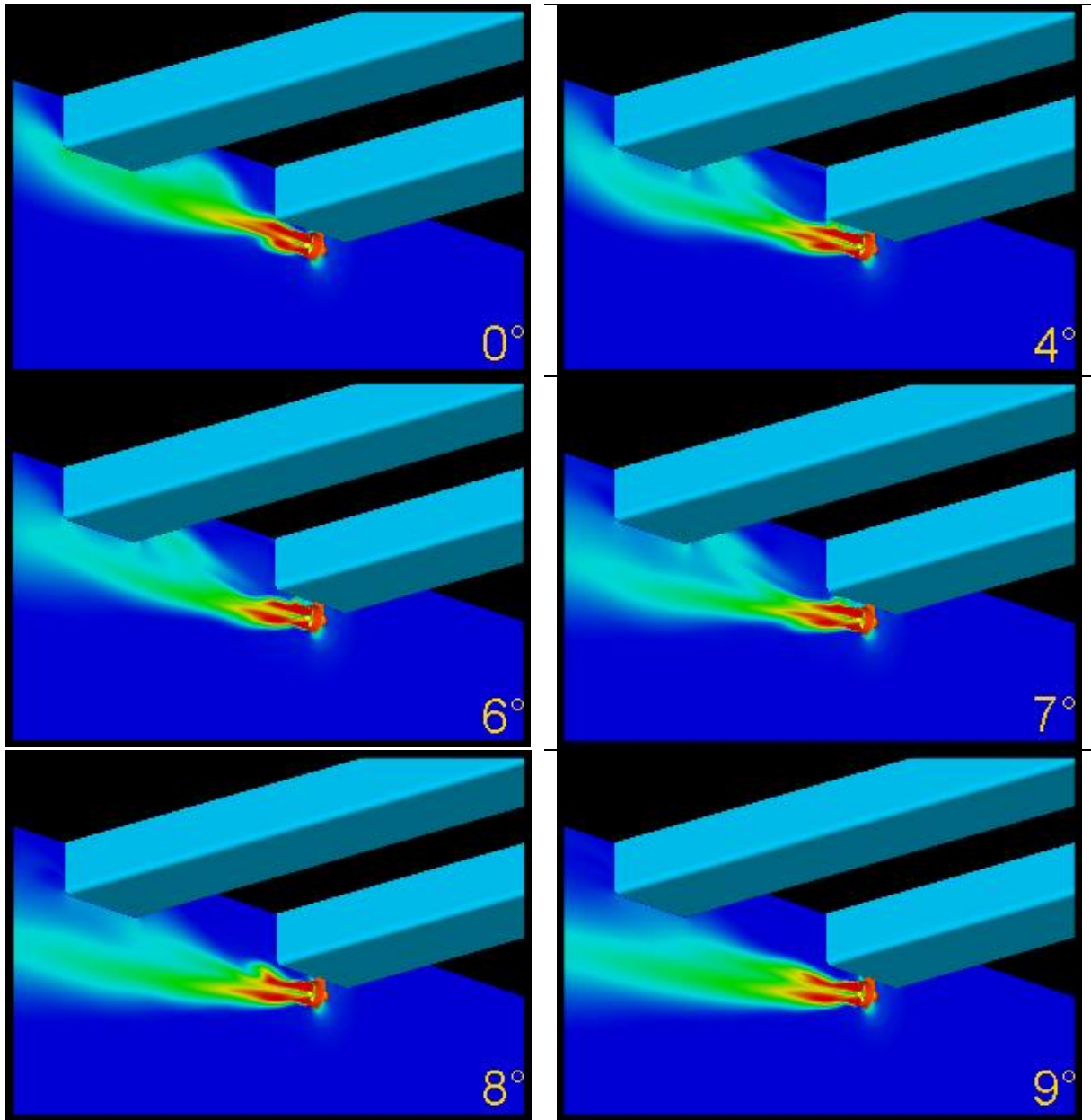
Fig. 5: Velocity distribution as a function of the tilt angle of the propeller axis
