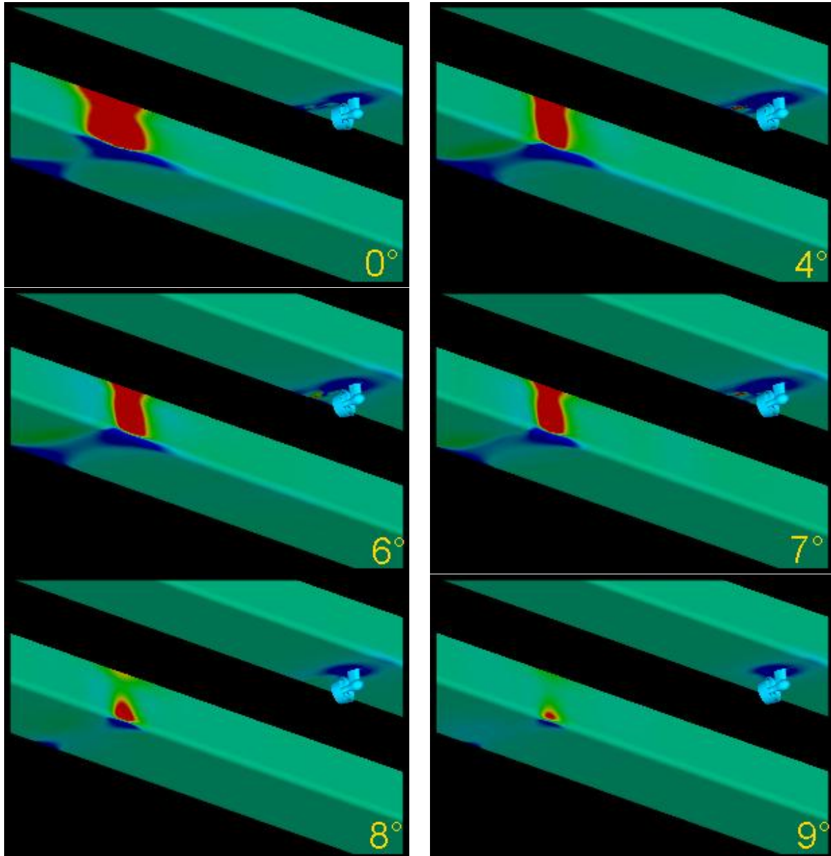
Fig. 8. Pressure distribution (showing the pressure side of pontoon 2)
