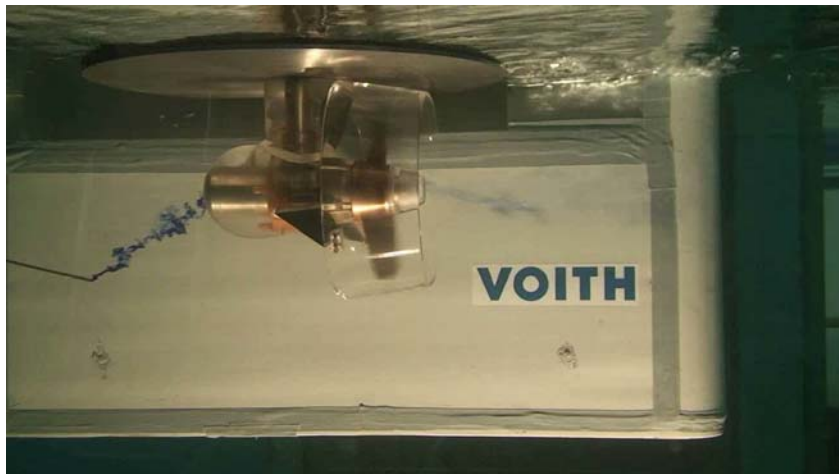
Fig. 16. Visualization of the flow pattern with ink
