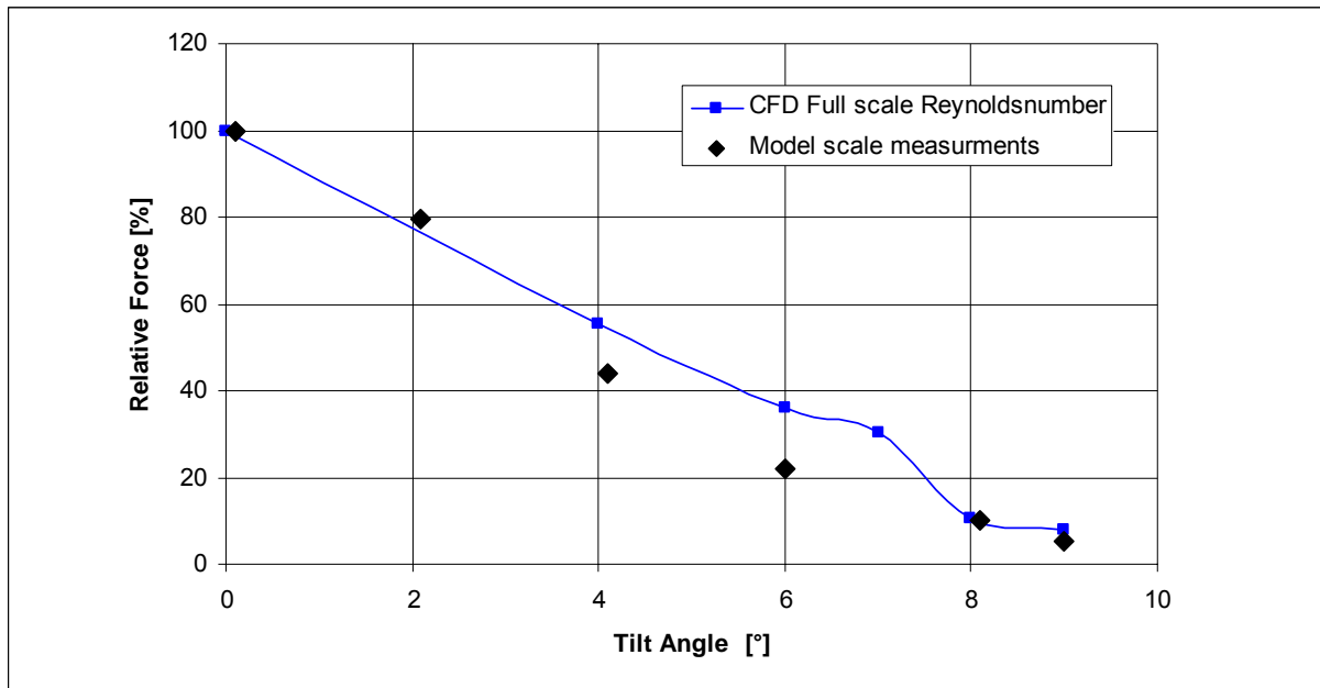
Fig. 15. Transverse forces, acting on pontoon 2; the maximum force on pontoon 2 is scaled as 100%; comparison of full scale CFD calculation and model test data
