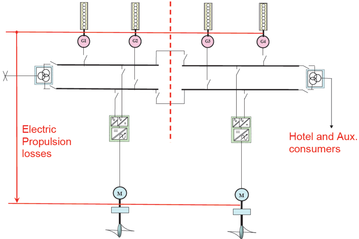
Fig 6. – LLC - Full Scale measurements of electric propulsion losses
