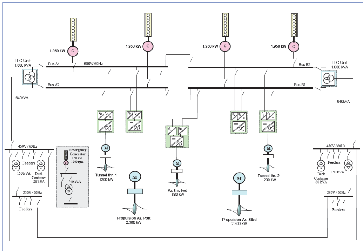
Fig 5. Viking Queen – Single line diagram
