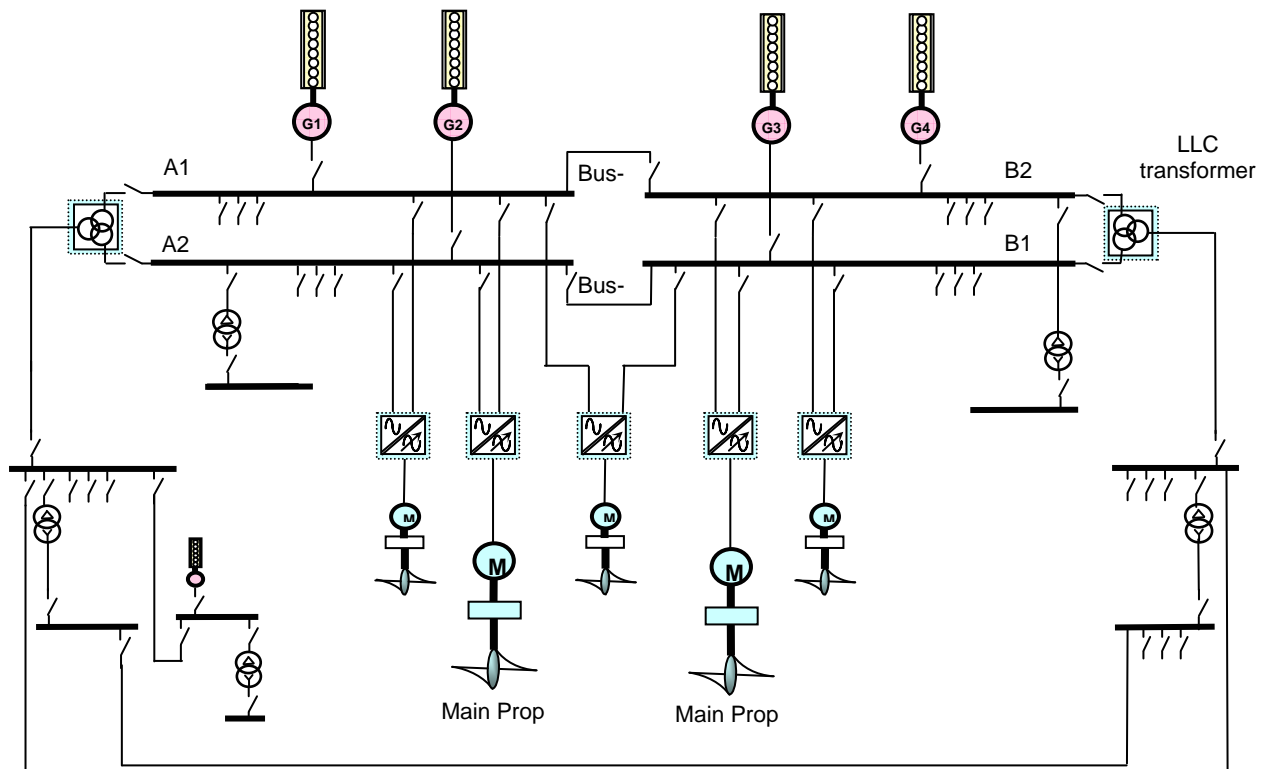
Fig.3. Typical DE system for OSV based on Low Loss Concept
