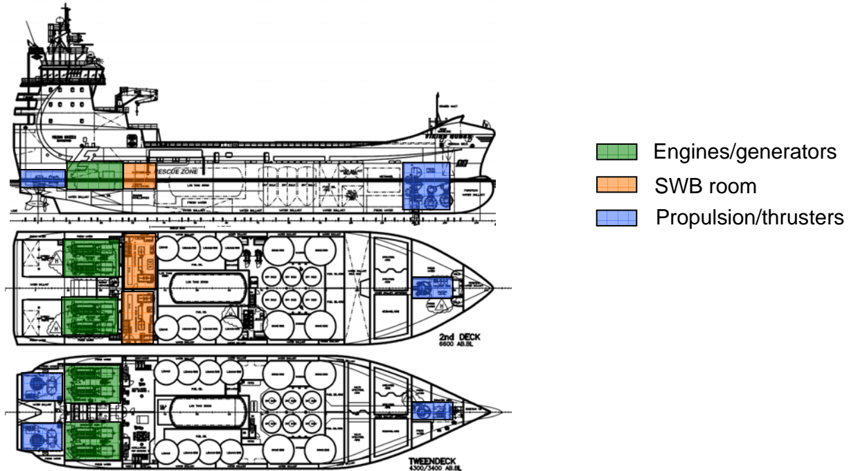
Fig 4. Viking Queen – Machinery and Propulsion arrangement
