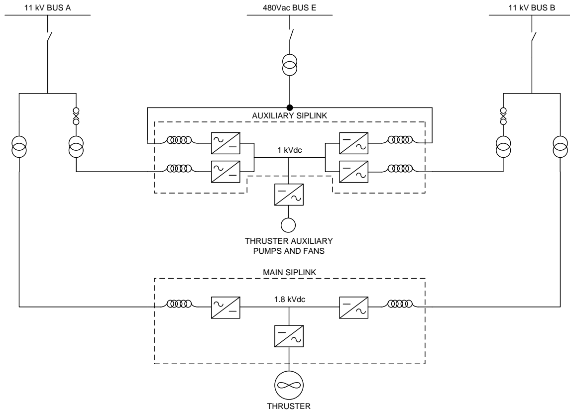
Figure 5-Arrangement of Main and Auxiliary Siplinks
