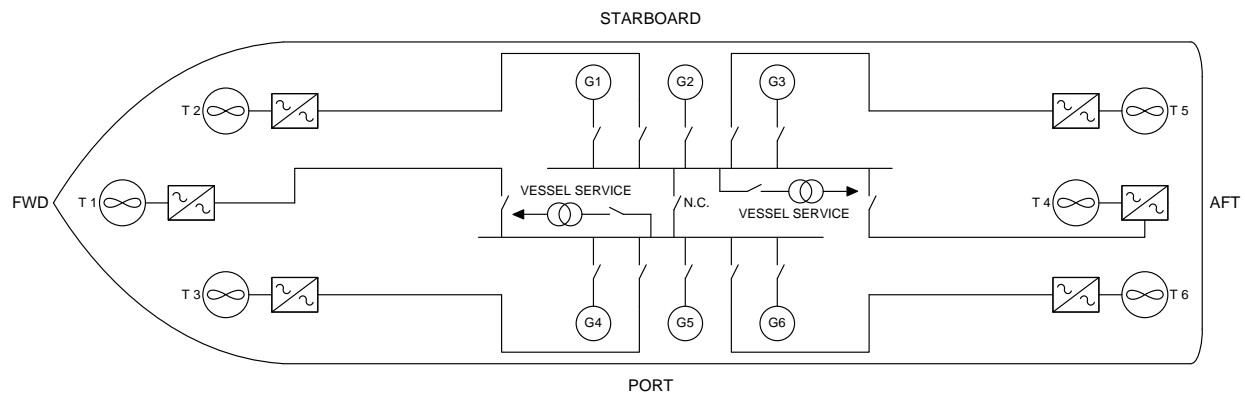
Figure 1 Conventional Propulsion System Arrangement
