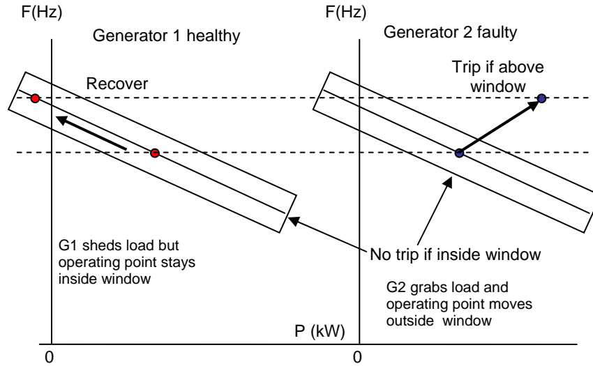
Figure 3-Identification of Faulty Generator
