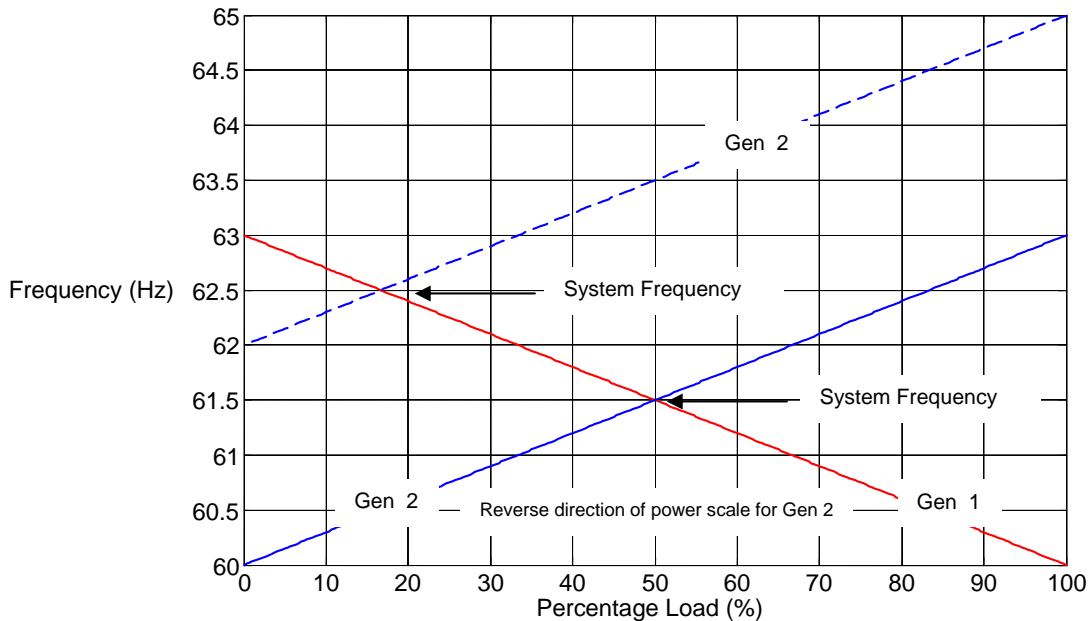
Figure 2- Generator Load Sharing by Droop
