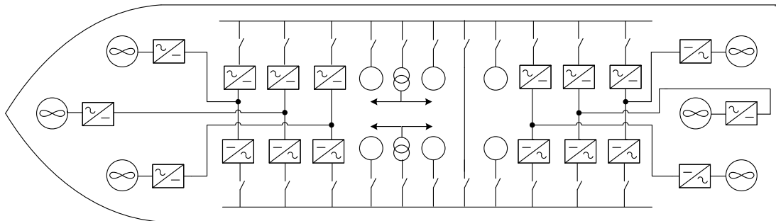
Figure 4-Arrangement of Siplink Based Propulsion System
