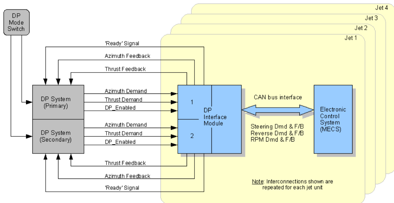
Figure 9- DP Interface to Jet Control System
