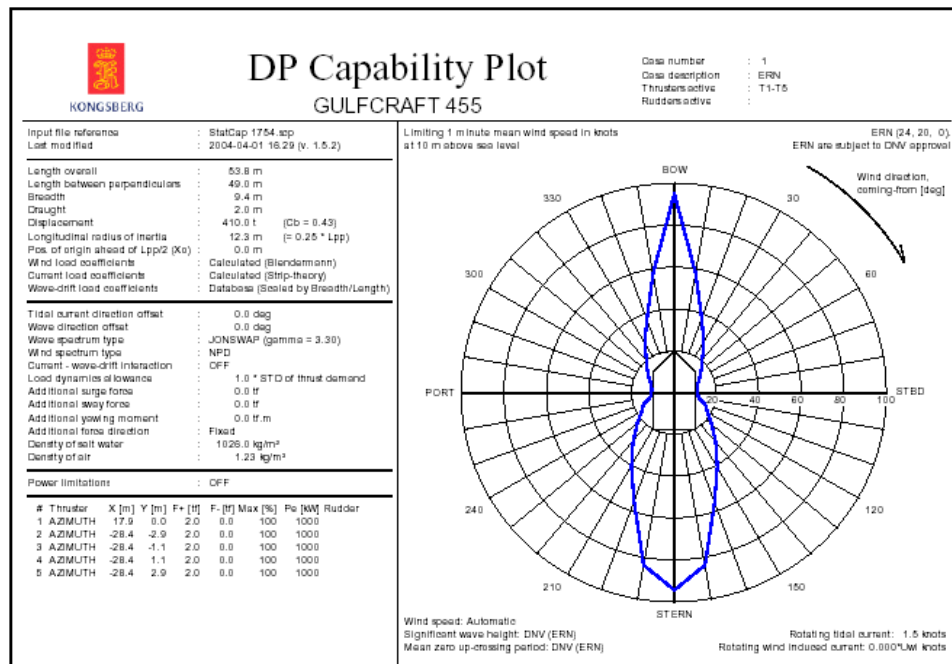
Figure 11- DP Capability Plot
