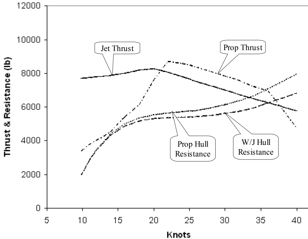
Figure 2- Waterjet vs Propeller Thrust Characteristics for a 35 Knot Vessel
