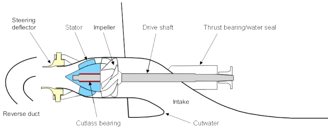
Figure 1 – Waterjet Key Components
