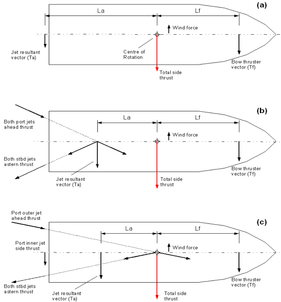
Figure 10- Transverse Thrust Methods for Quadruple Waterjets
