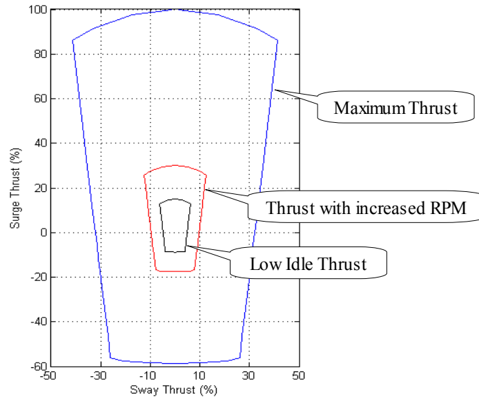
Figure 8- Jet Manoeuvring Thrust Variation with Engine Speed
