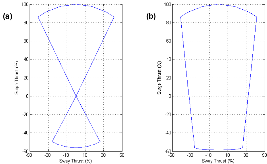
Figure 6- Thrust Envelopes for Steering-Mounted and Split Duct Reverse
