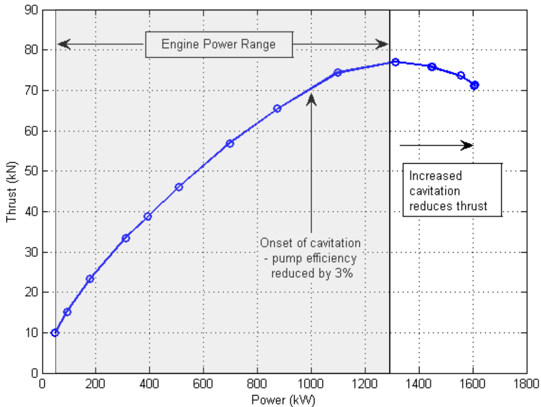
Figure 5- HM811 Bollard Pull Thrust vs Power
