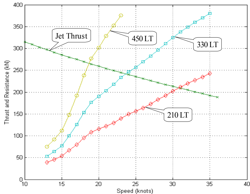
Figure 4- Waterjet Crew Boat Speed at Different Loading Conditions
