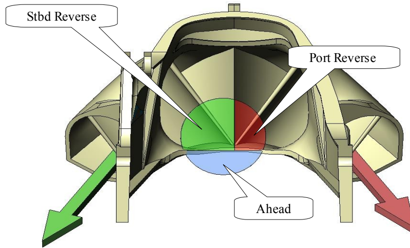
Figure 7- View into Reverse Duct along Jet Stream
