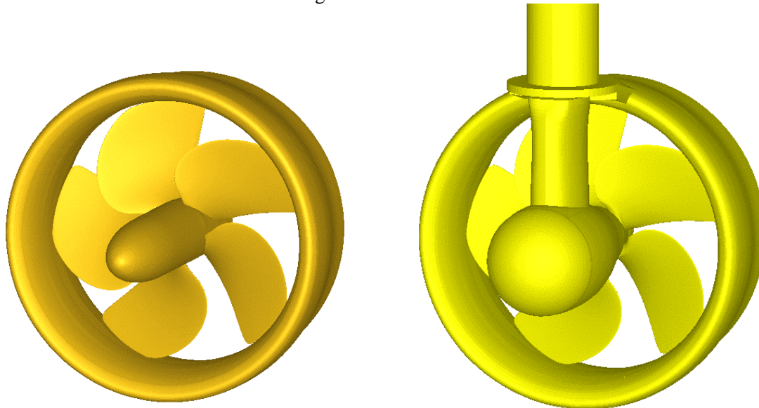
Figure 7: Comparison of test-hub configuration (left) and thruster unit
