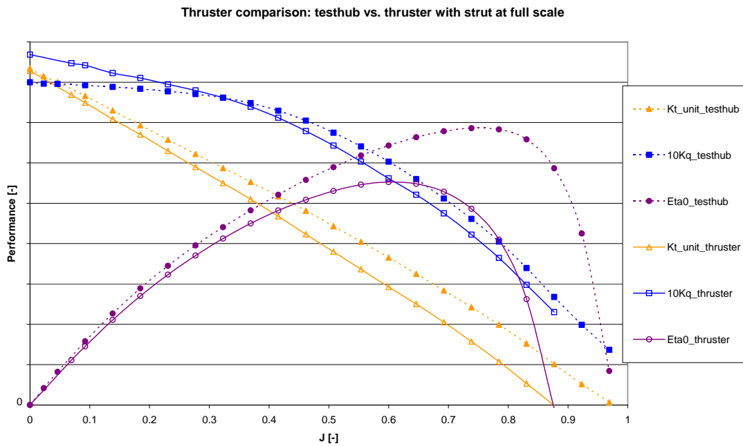
Figure 8: Comparison of open water performance of test-hub configuration (dotted lines) and thruster unit (solid lines) for full scale
