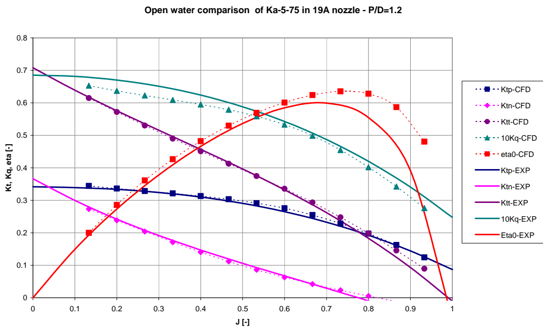
Figure 2: open water performance comparison of Ka5-75 in 19A nozzle
