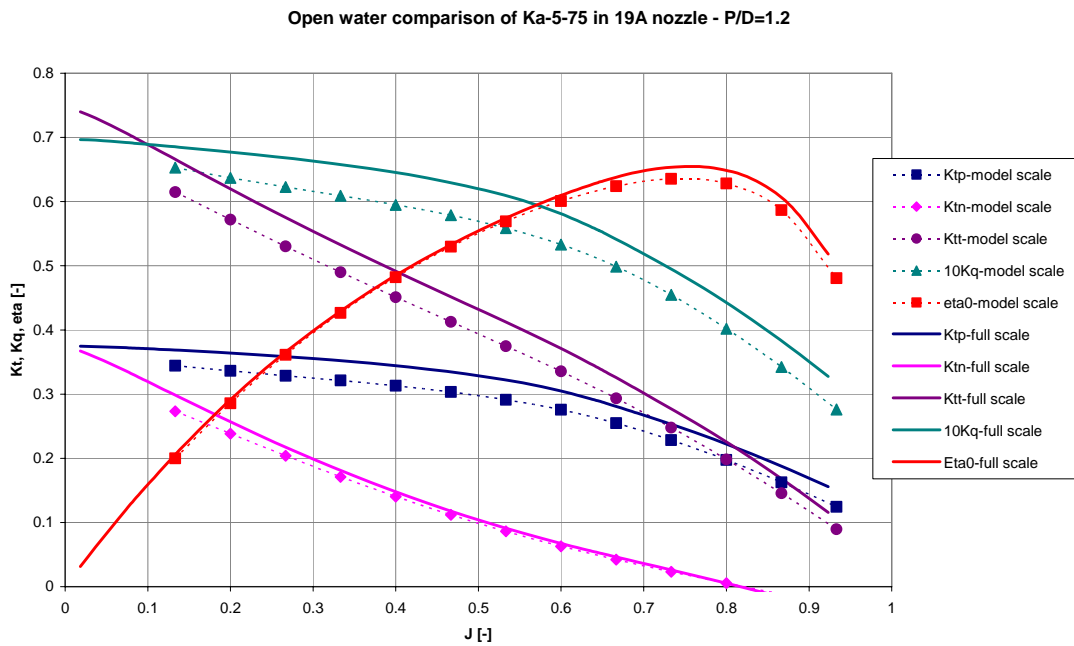
Figure 4: Comparison of open water performance of Ka5-75 propeller in 19A-nozzle on model scale and full scale.
