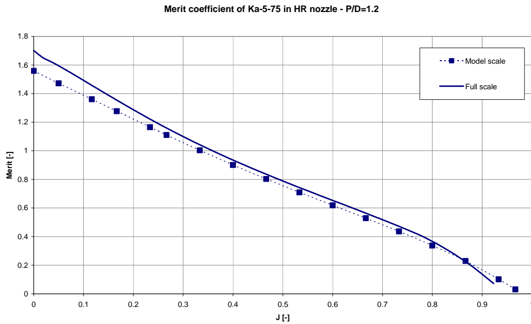
Figure 6: Merit coefficient of Ka5-75 propeller in HR-nozzle on model scale and full scale.
