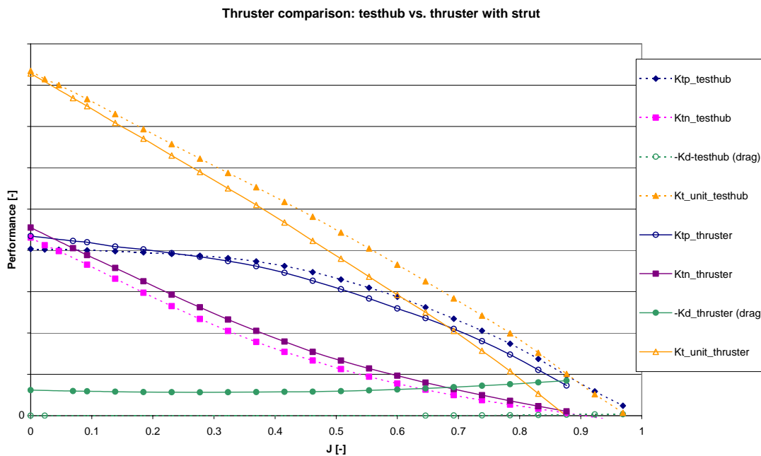
Figure 10: Comparison of propeller, nozzle and unit thrust of test-hub configuration (dotted lines) and thruster unit (solid lines)
