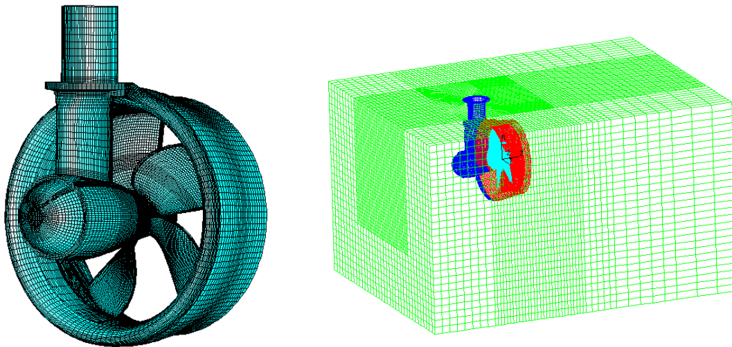
Figure 1: Example of surface mesh of complete thruster unit (left) and mesh of numerical domain.
