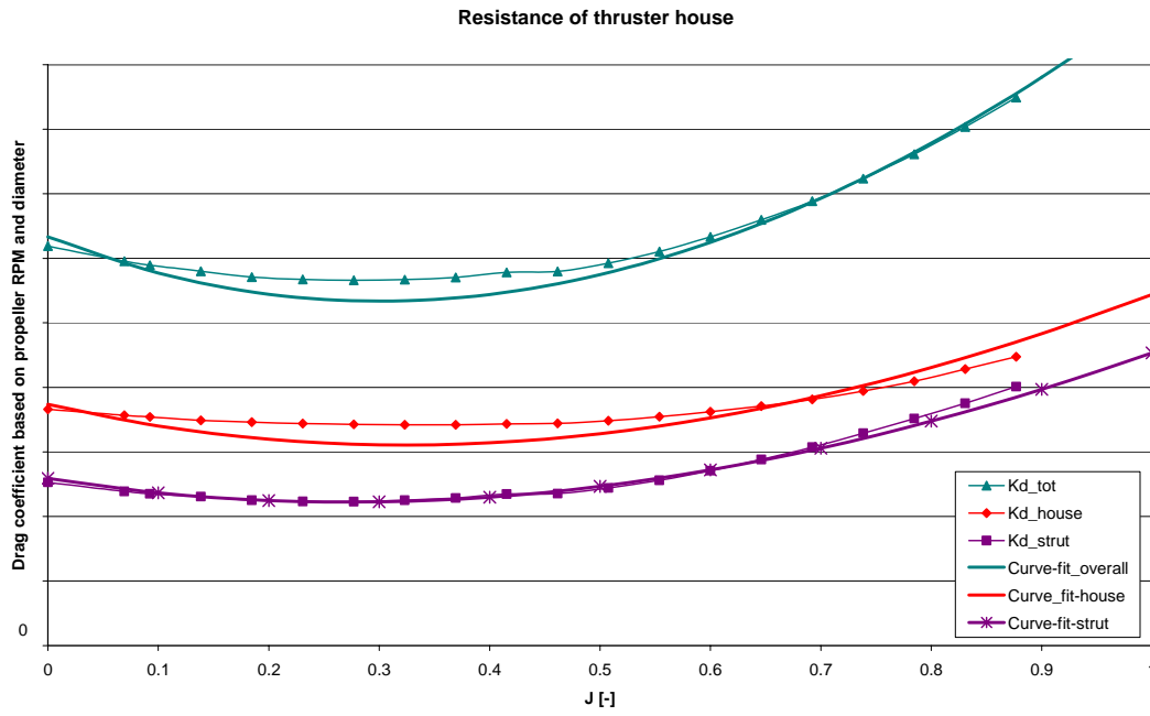
Figure 11: Analysis of thruster house and strut drag components
