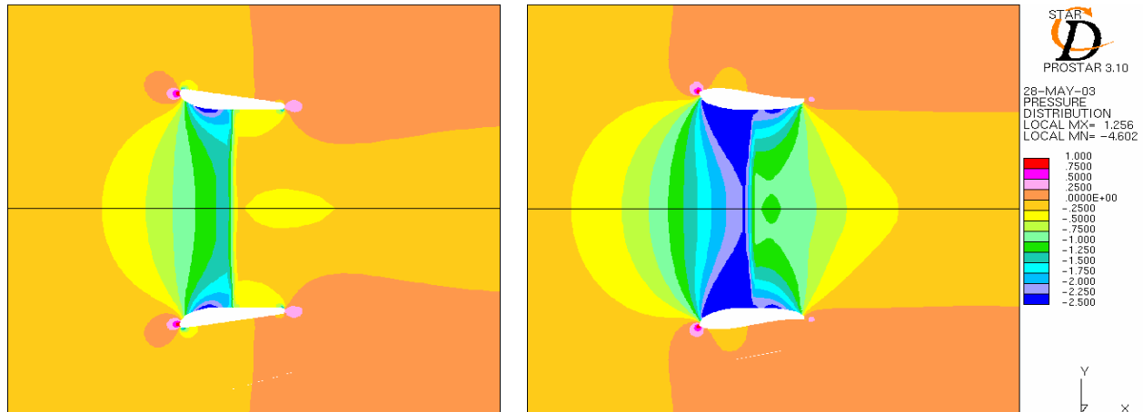
Figure 3: Comparison of 19A (left) and Lips-HR nozzle cross-sectional profile. Contours indicate pressure distribution in free-sailing condition
