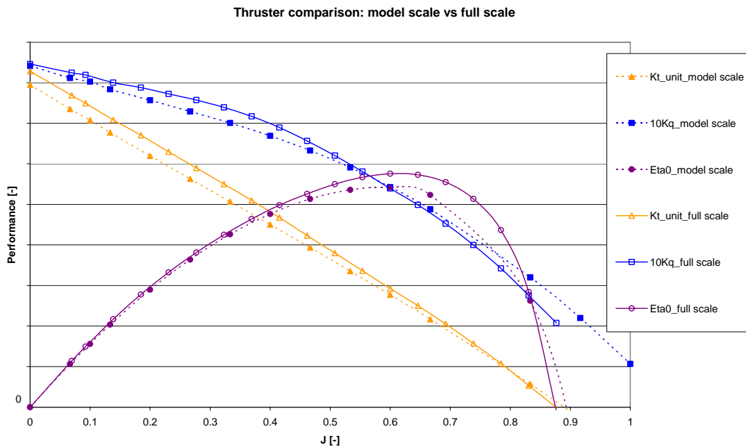
Figure 9: Comparison of open water performance of model scale thruster unit (dotted lines) and full scale thruster unit (solid lines)
