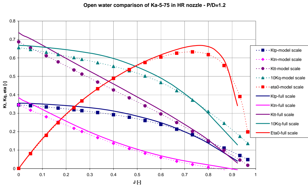
Figure 5: Comparison of open water performance of Ka5-75 propeller in HR-nozzle on model scale and full scale.
