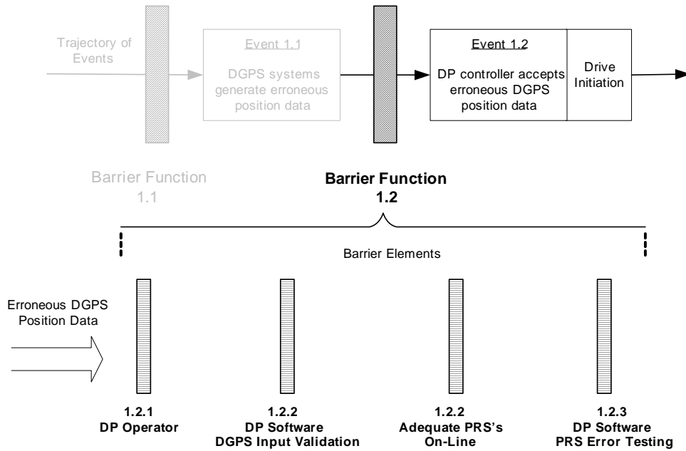
Figure 6: Barrier Elements to Prevent DP Controller Using Erroneous DGPS Data
