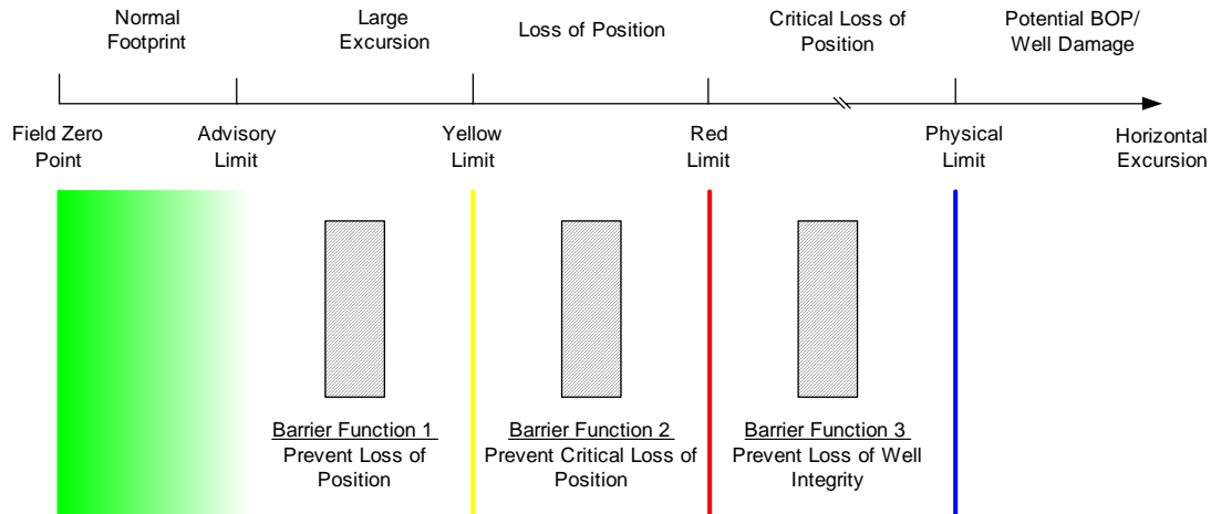
Figure 3: Three Main Barrier Functions with Respect to the Safety of DP Drilling Operation
