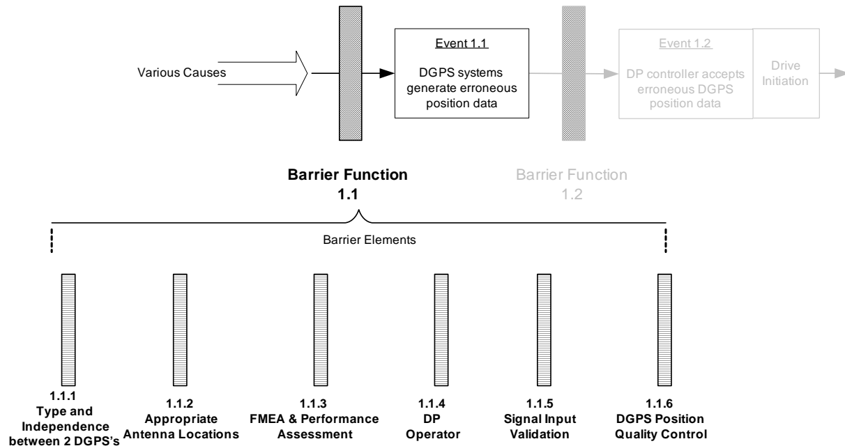
Figure 5: Barrier Elements to Prevent Erroneous Position Data from DGPS
