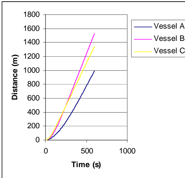
Figure 2: DP vessel Drifting Rates
