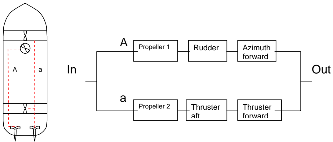
Figure 5, Functional diagram and reliability block diagram with main systems for redundant PK
