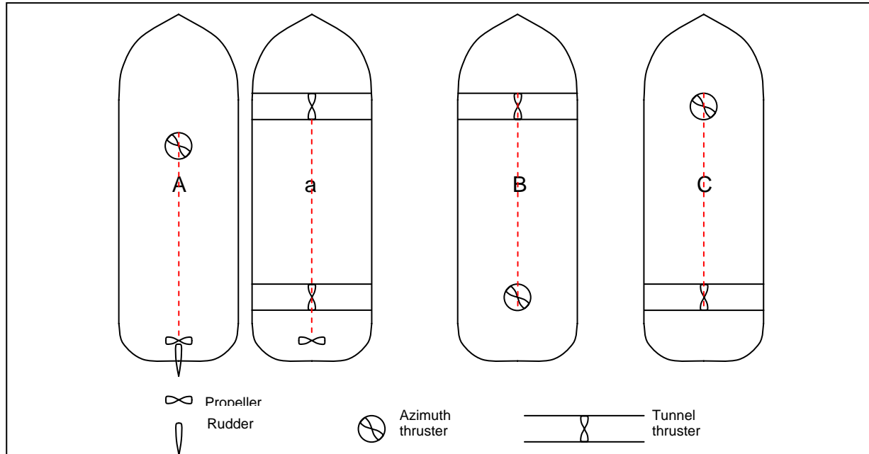
Figure 1 - Minimum thruster/propulsion configurations for position keeping
