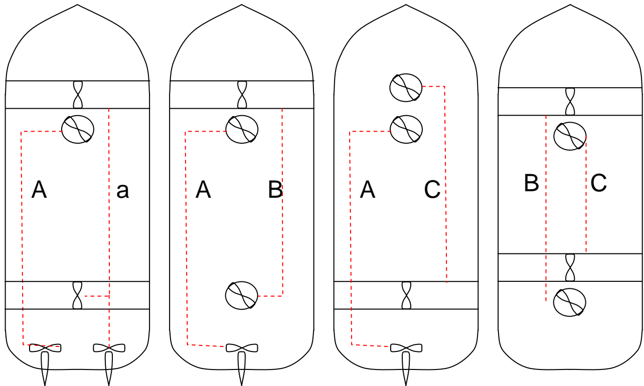
Figure 2 Example on thruster configurations for technical redundancy
