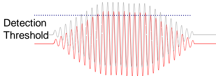
Received & Filtered Pulse
