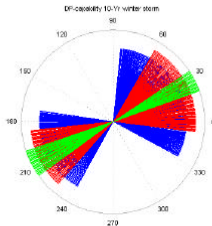
Figure 6. DP-capability plot for 10-Year winter storm condition
