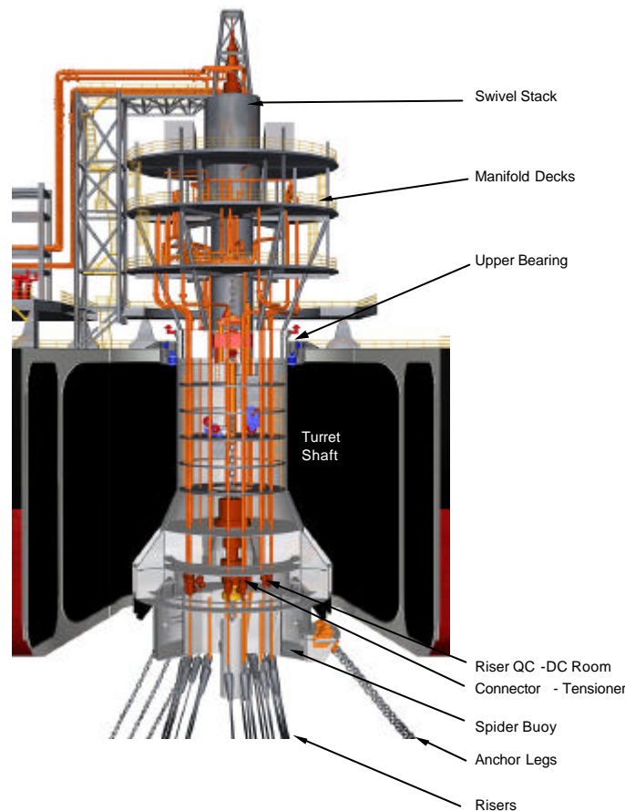
Figure 3. The Terra Nova disconnectable turret mooring system
