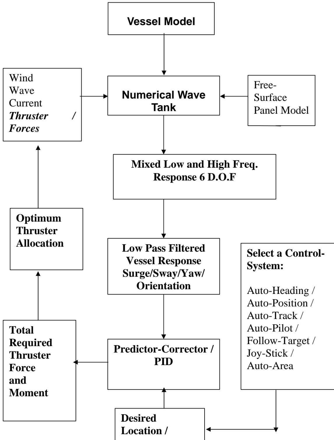
Figure 1 Numerical Wave Tank Simulation of DP System
