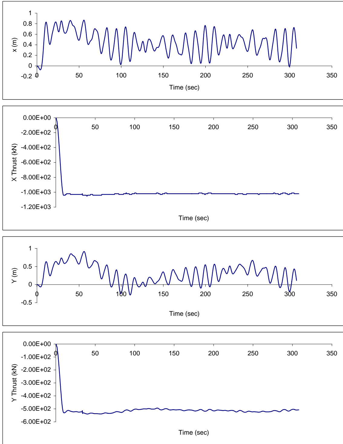
Figure 6. Surge and sway displacements and thrust, H_s=4\text{m} , wave heading 45 deg., current of 1m/s with an (approximate) heading of 30 deg.
