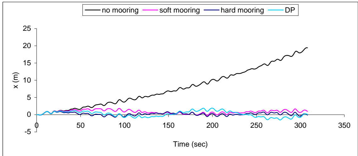
Figure 3. Surge displacements for different mooring and DP; H_s = 4m. , heading=0 deg.
