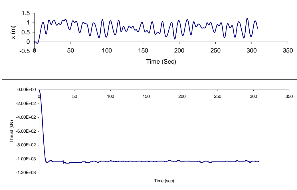
Figure 5. Surge displacement and DP thrust; H_s = 4\text{m} , heading = 0\text{deg.} , current = 1\text{m/s} , initial steady mean thrust of 1000\text{ kN} .
