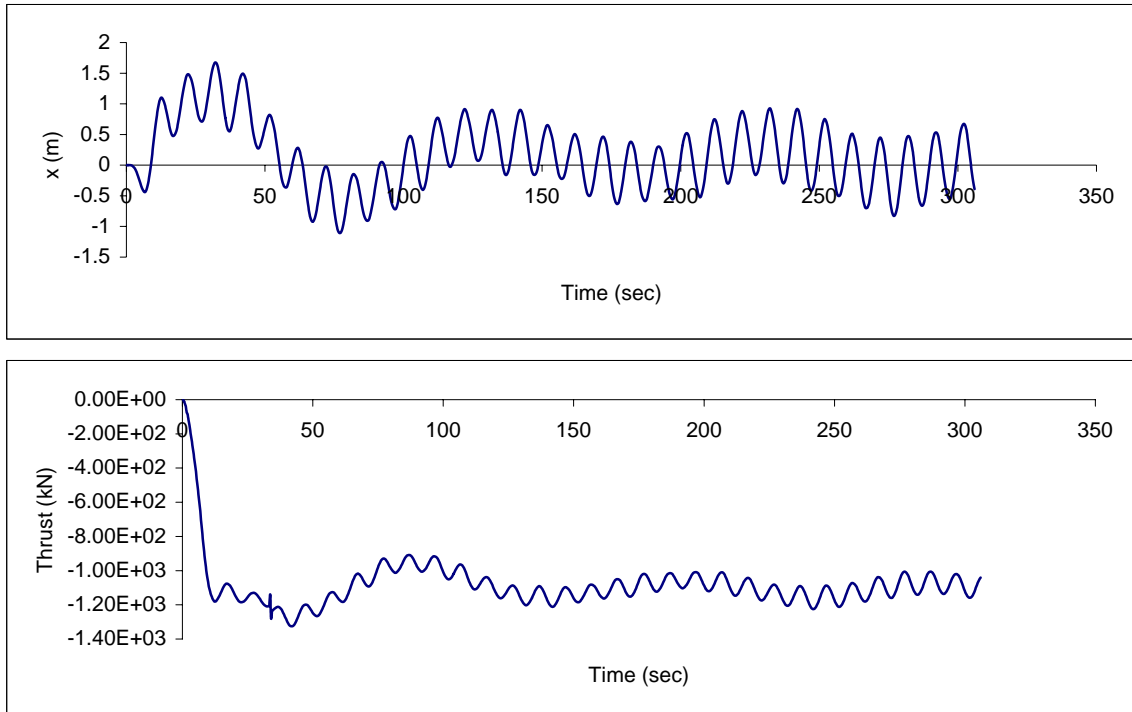
Figure 7: Surge displacement and thrust for a very steep nonlinear regular wave of period 10 sec. And height 10 m, wave heading 0 deg., current 1m/s.
