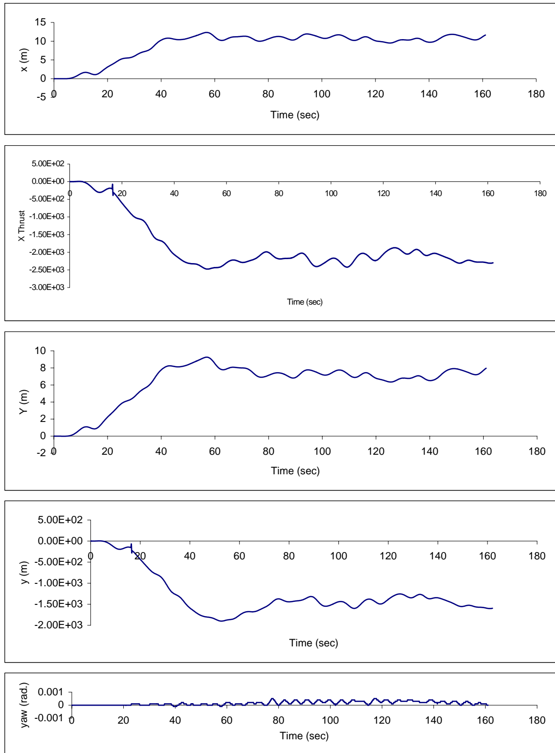
Figure 9. Surge, sway and yaw displacements and D thrust for the triangular semi submersible; H_s=6m , heading = 45 deg., current 1m/s with heading 30 deg.
