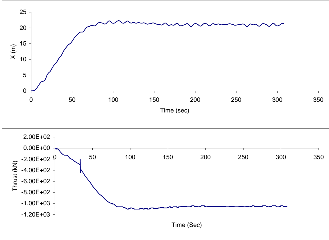
Figure 4. Surge displacement and DP thrust; H_s = 4\text{m} , heading = 0\text{deg.} , current = 1\text{m/s} , no initial steady mean thrust .
