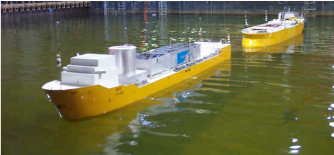
Figure 5: Model test of DP controlled FPSO and offloading tanker.
