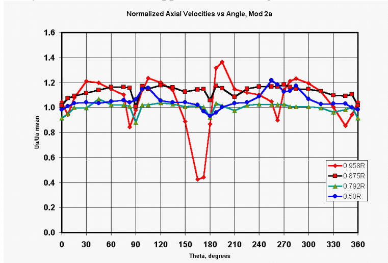
Figure 9: Air Test Normalized Axial Velocity - Mod 2
