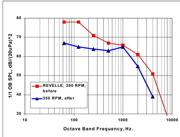
Figure 17: Room 2-22-2, 350 RPM, SPL Spectra Before & After
