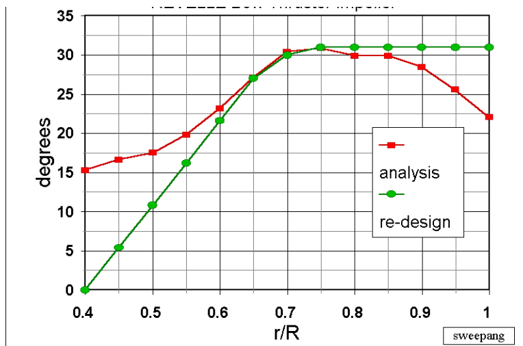
Figure 12: Leading Edge Sweep Angle vs Radius
