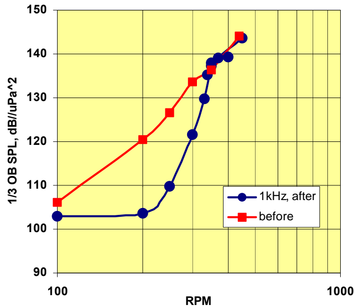
Figure 15: Underwater Noise-REVELLE Bow Thruster
