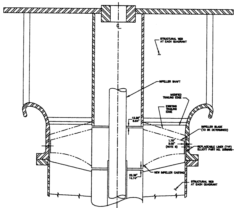
Figure 6: Thruster Modifications
