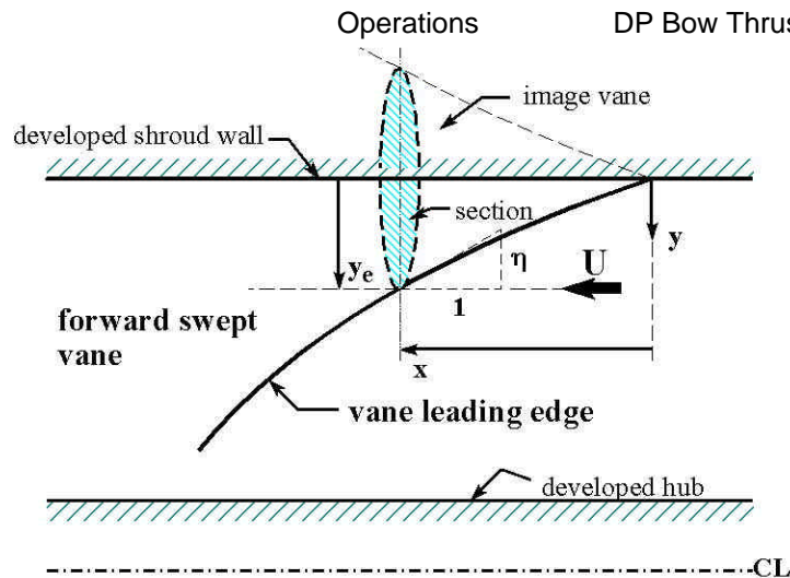
Figure 11: Forward Swept Blade (Vane) Showing Radial Section
