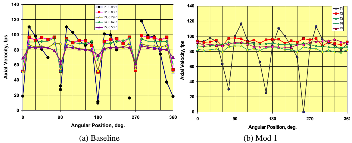
Figure 5: Air Test Axial Velocity
