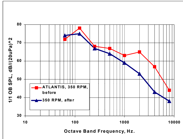
Figure 3: Room 2-22-2, Before and After SPLs, 350 RPM - ATLANTIS
