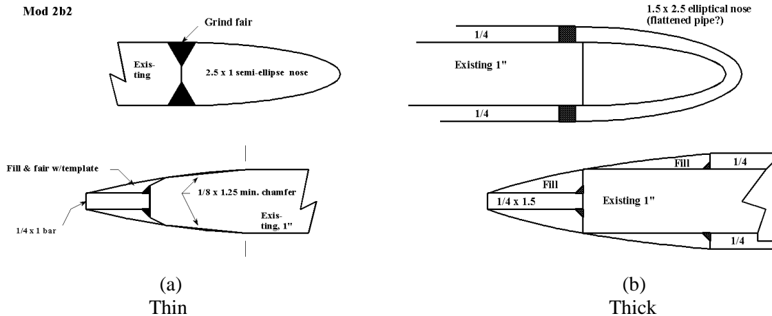
Figure 7: Plate Fairing
