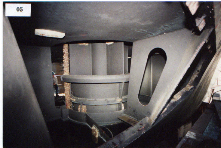
Figure 2: Thruster Sea Chest (ATLANTIS)
