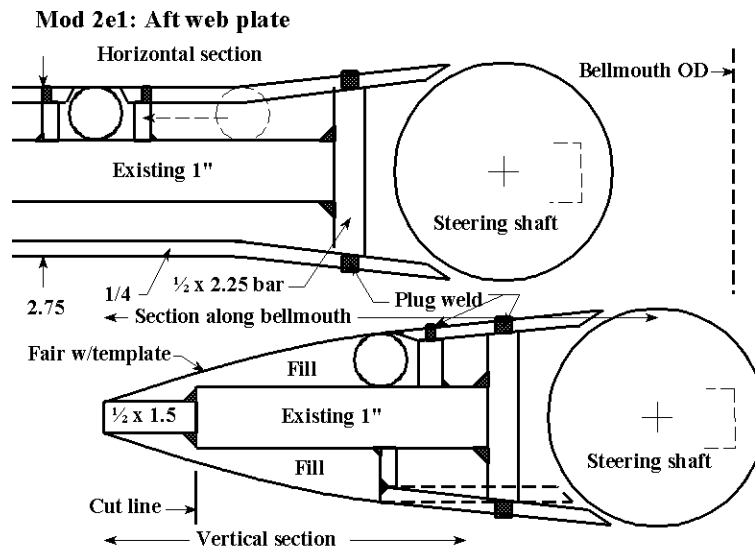
Figure 8: Steering Shaft Fairing-First Design for Air-Test
