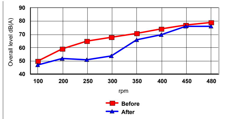
Figure 16: Room 2-22-2 Overall Noise Levels, REVELLE
