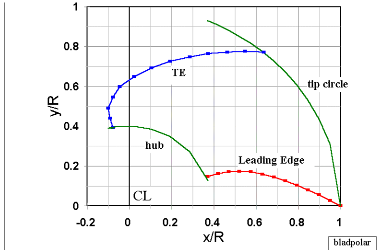
Figure 13: Axial Projection - Forward Skewed Blade
