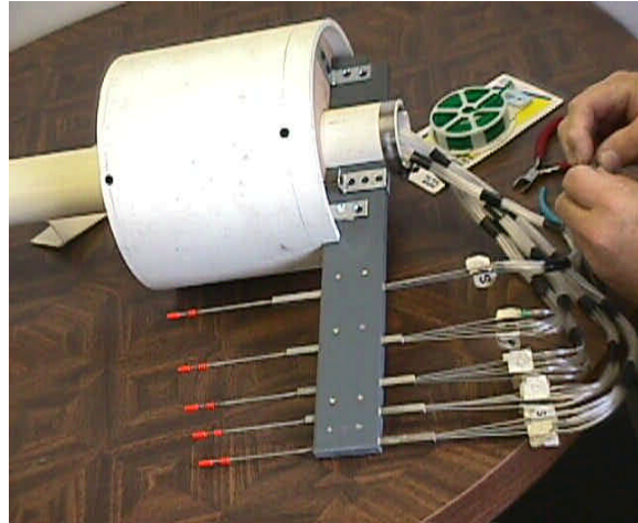
(c) Pitot Rake
