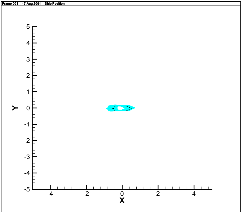
Fig. 14 Ship trajectory due to the long-term random disturbance (with control)
