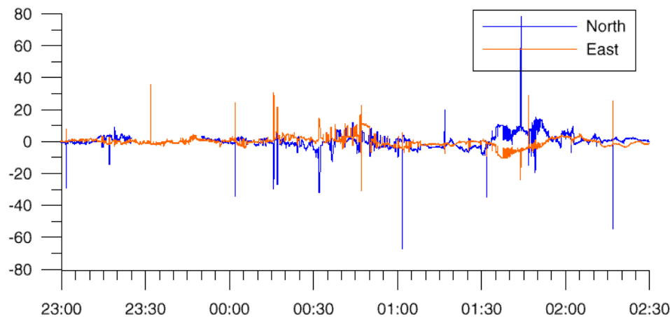
Figure 9. Single Frequency DGPS, Macae – Rio (80 km)
