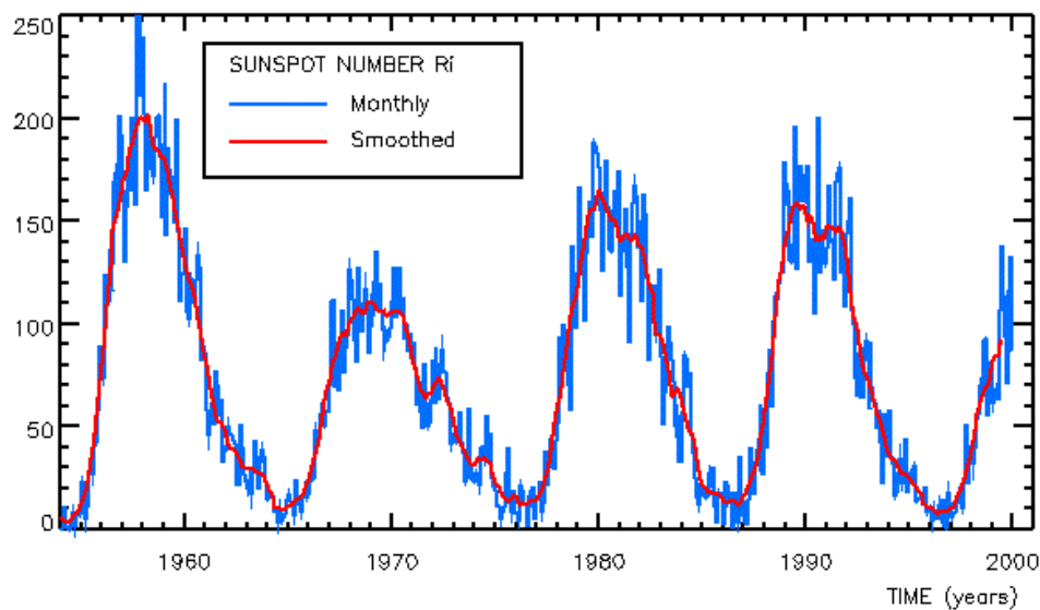
Figure 2. Historic Sunspot data
