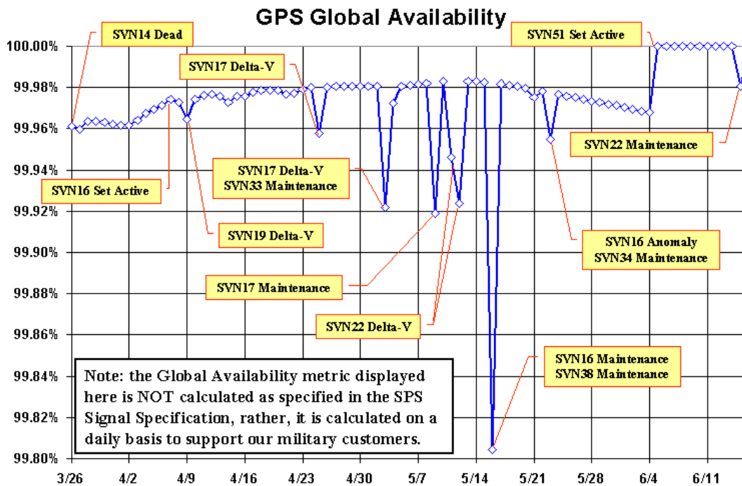
Figure 6. Global GPS Availability (March 26 to June 16 2000)
