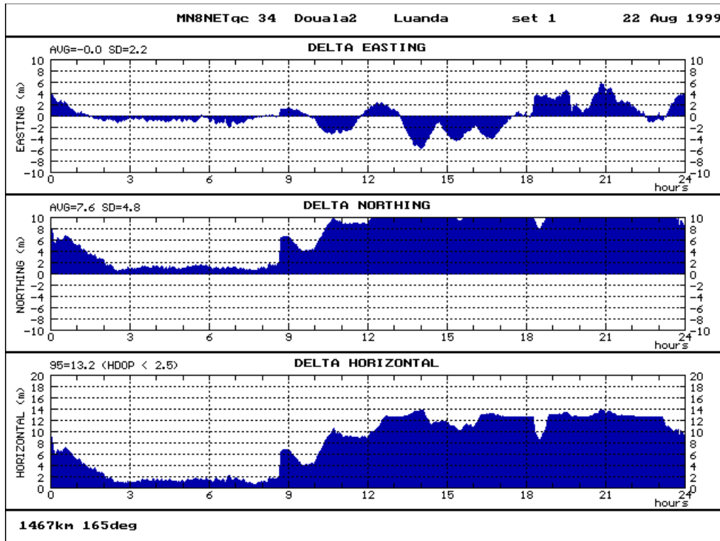
Figure 4. Single Frequency DGPS. Douala/Luanda 22.08.99
