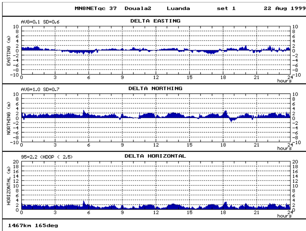
Figure 5. Dual frequency DGPS. Douala / Luanda, 22.08.99
