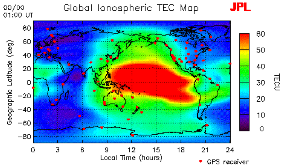
Figure 3. Ionospheric TEC Map
