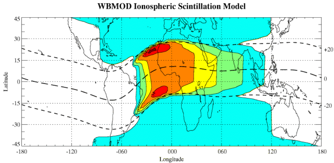
Figure 8. Ionospheric Irregularities (scintillations)
