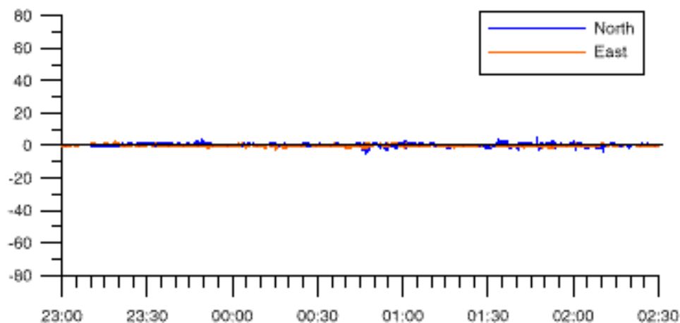
Figure 10. Dual frequency DGPS+DGLONASS Multiref, Macae – 2*Rio (80 km) / Recife (1870 km)
