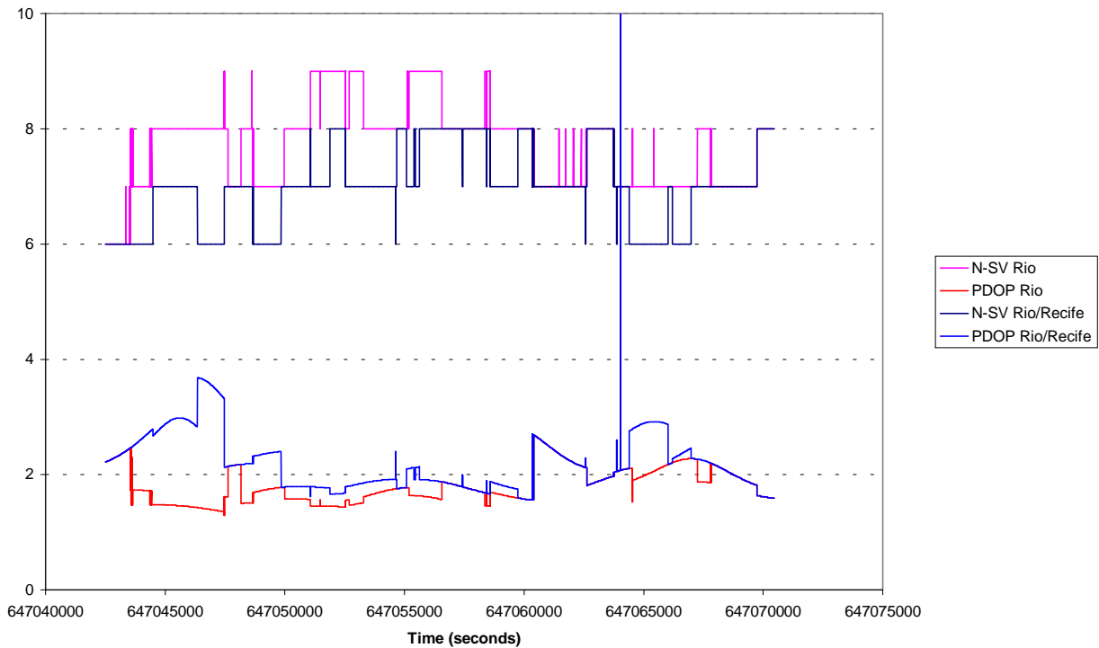
Figure 7. Satellite Geometry for Rio and Rio/Recife
