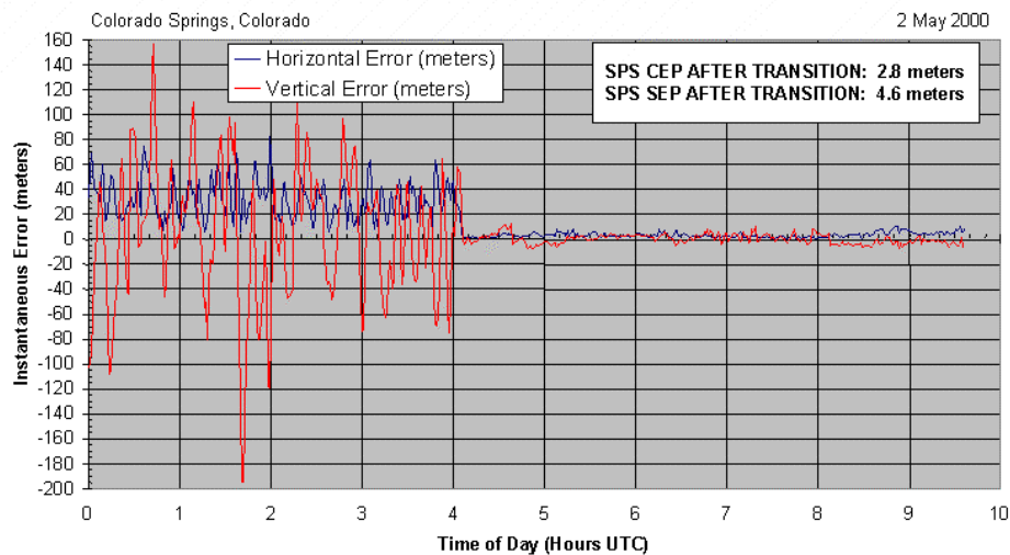
Figure 1. SA Transition: Accuracy Improvement in Colorado Springs. (CEP: 50% horizontal accuracy. SEP: 50% 3-dimensional accuracy)
