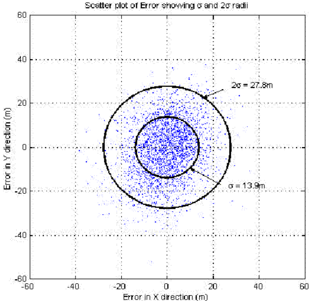
Figure , Sea Trial 1 - Position Scatter Plot in 3200 m
