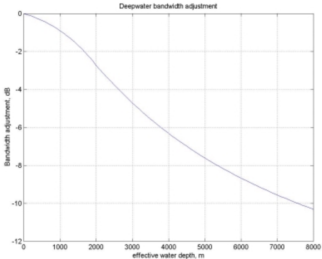
Figure – Bandwidth reduction with Water Depth
