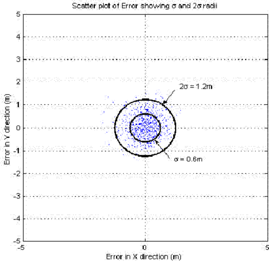
Figure Sea Trial 2 – Position Error in 580 m
