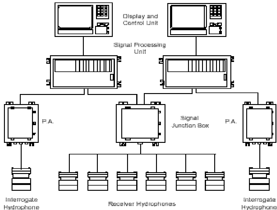
Figure 9. System Architecture
