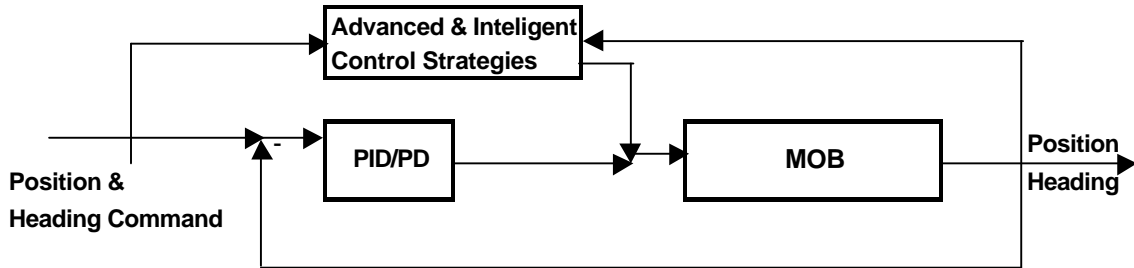
Figure 6 Parallel Alternate Controls
