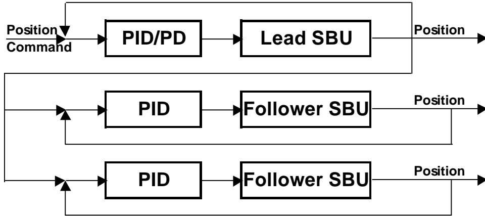
Figure 6 Parallel Alternate Controls
