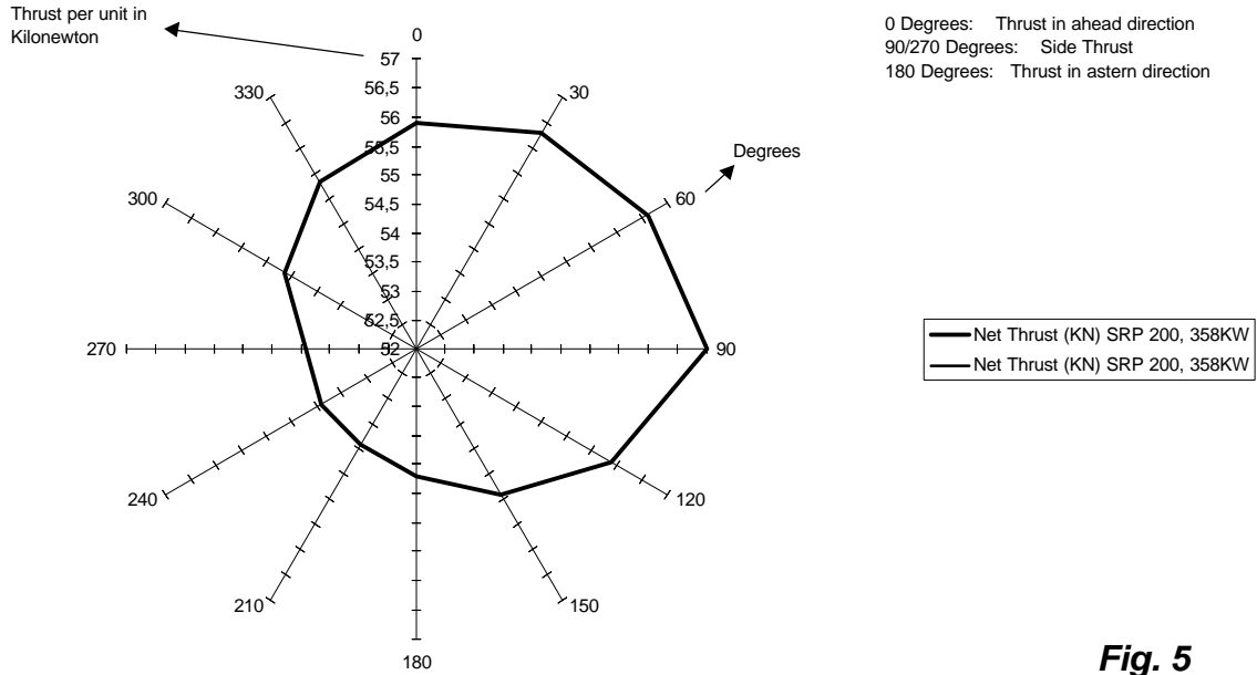
SEA 1052, 220 ' Ferry, Polar Diagram of Net Thrust for Schottel Twin Propeller 700 KW and Conventional Propulsion 1020 KW
