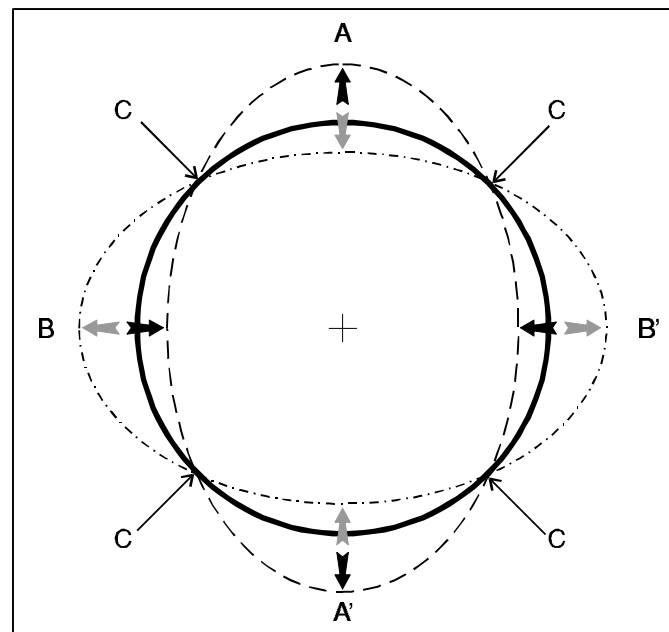
Fig 7. Graphic of a Vibrating structural gyro
