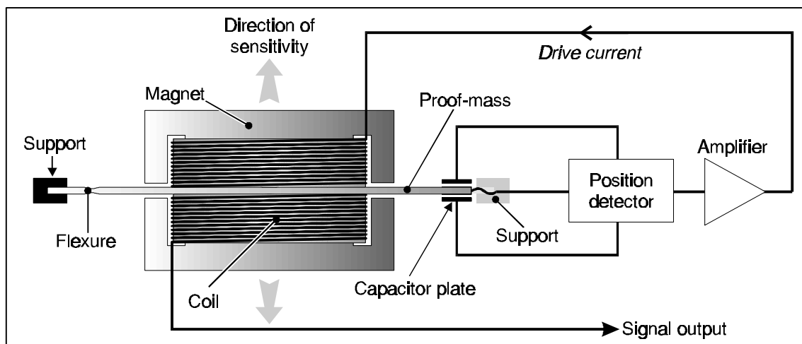
Fig 6. Graphic of an Accelerometer
