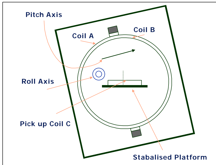
Figure 5. Fluid Stabilized Measurement Platform
