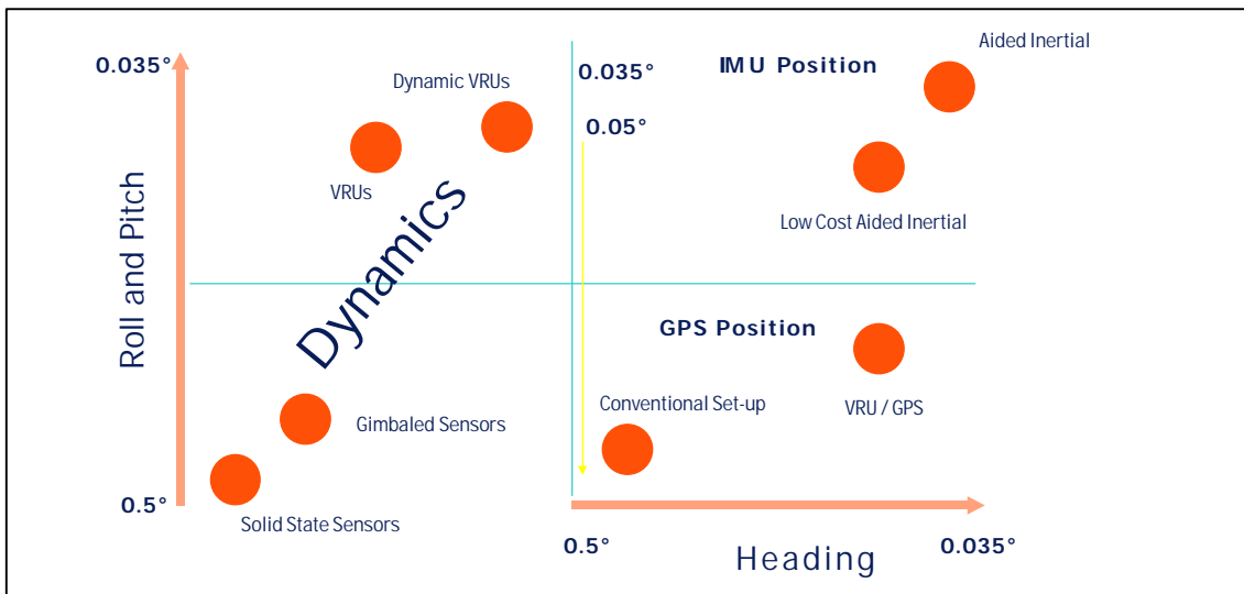
Figure 3 Contribution to correction of overall Error Budget
