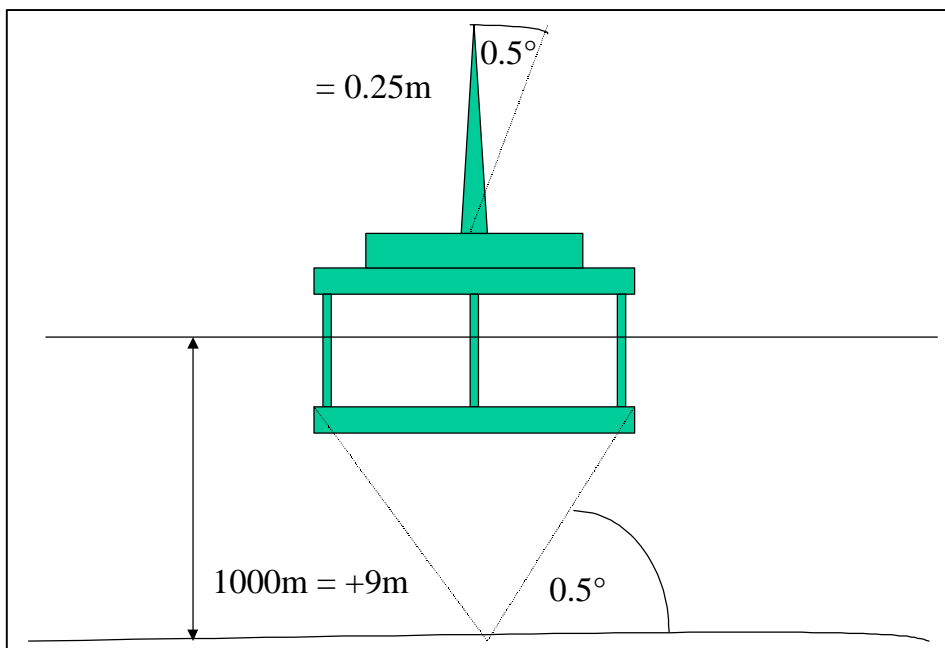
Figure 1. GPS and Acoustic Error Budget due to Roll Error
