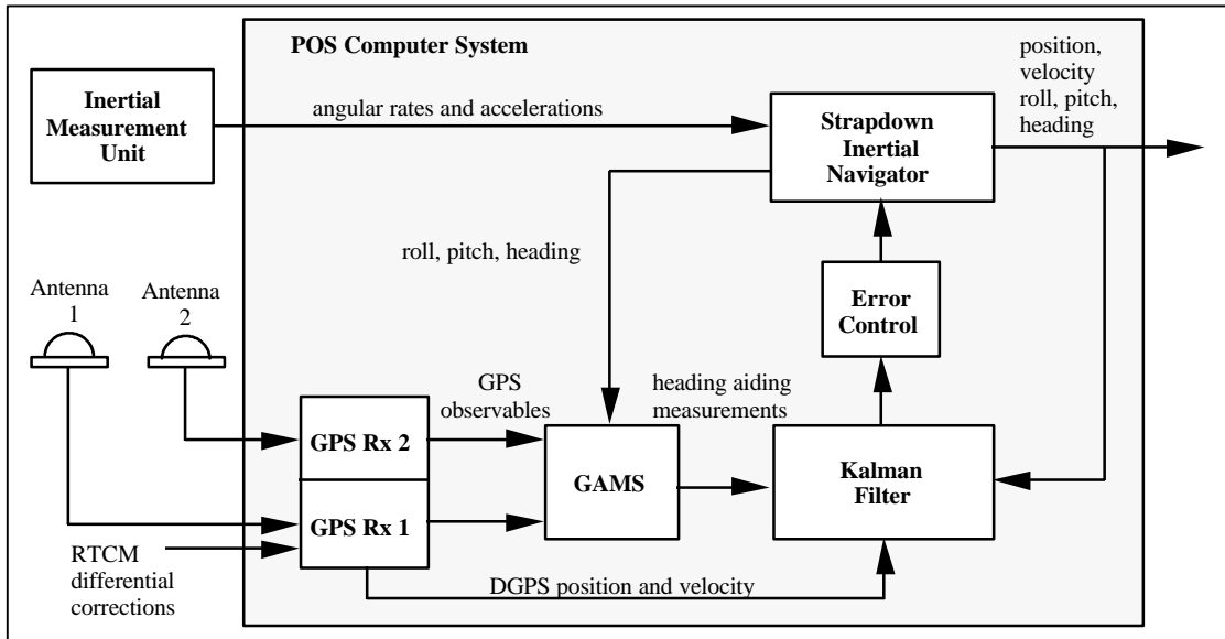
Fig 9. The TSS POS MV Functional Layout
