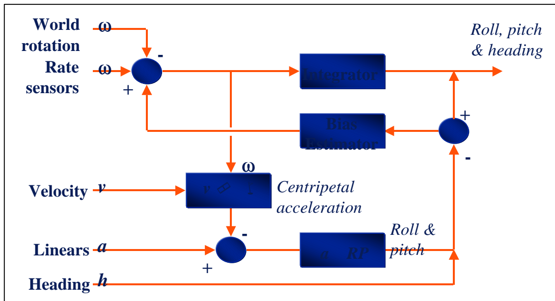
Fig 8. DMS Algorithm
