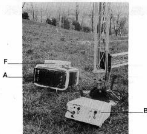
FIG. 8 - BEACON (B) - BOOSTER AMPLIFIER (A) AND L.D. FILTER (F) FOR A SYLEDIS L.D.
