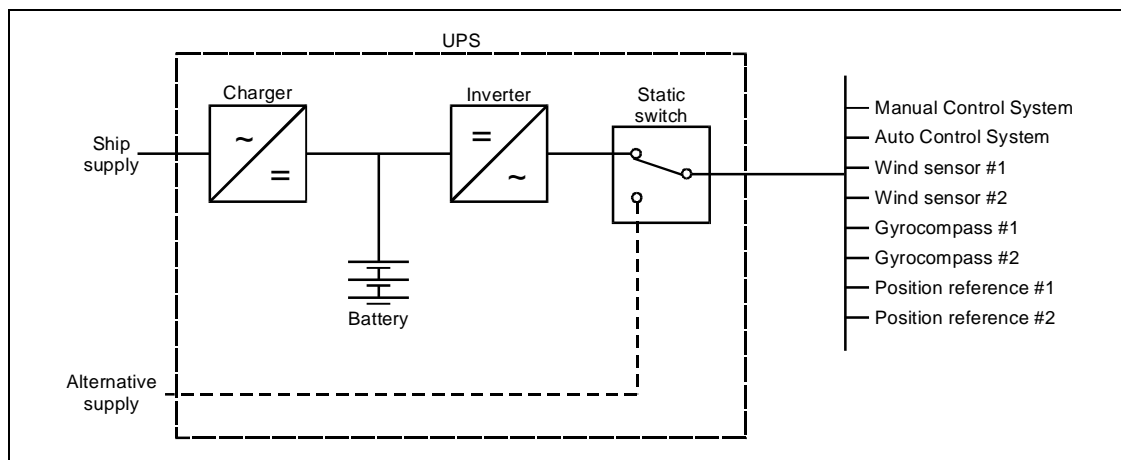
Figure UPS1: Simple UPS Suitable for DPS-1
