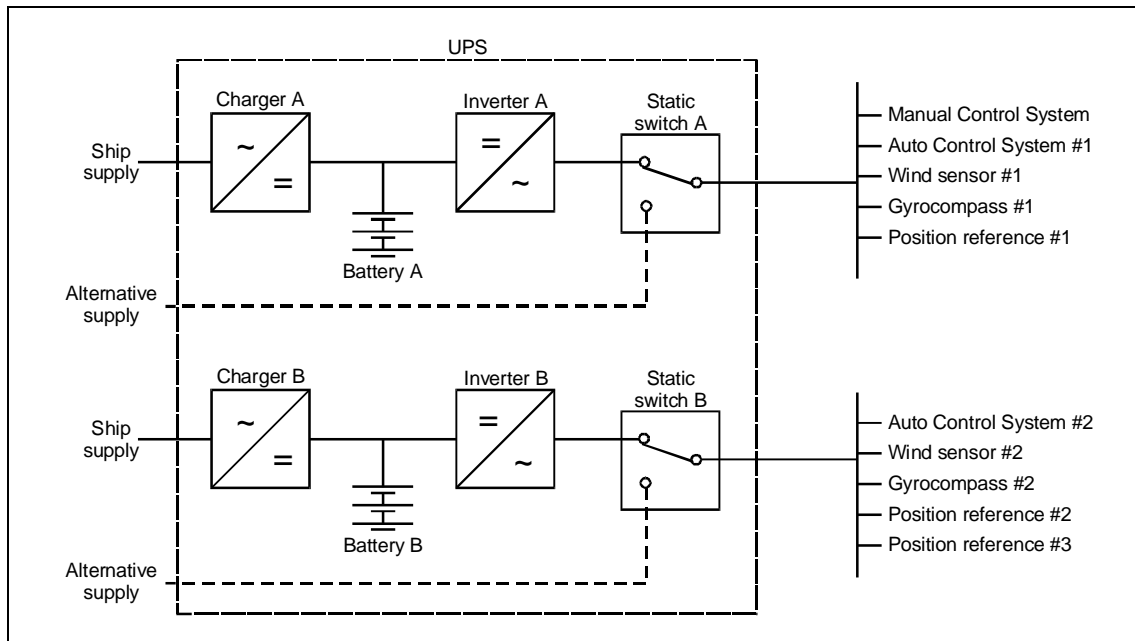
Figure UPS2: Redundant UPS suitable for DPS-2
