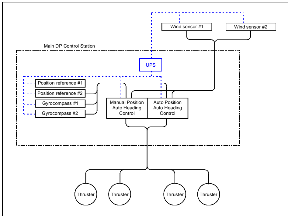
Figure DPS1: Example DPS-1 Control System Arrangement
