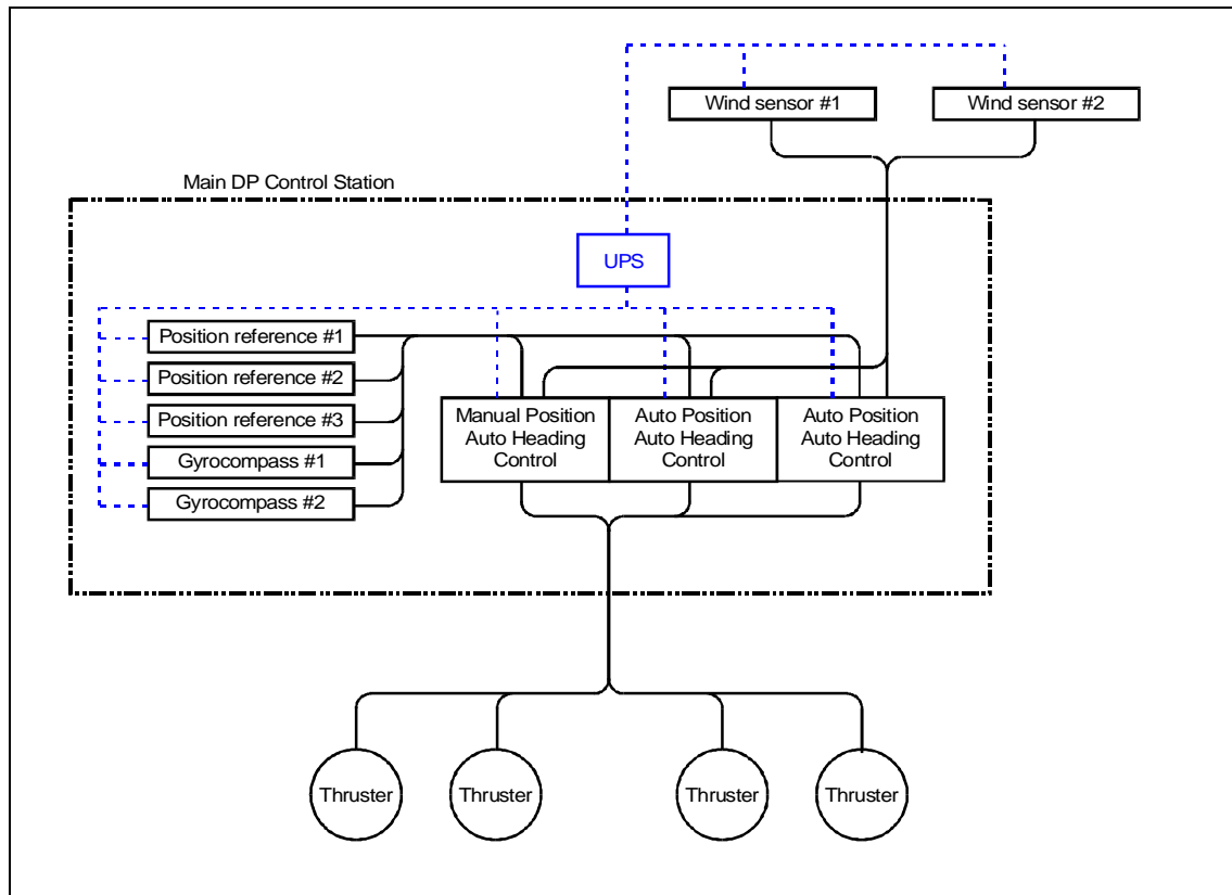
Figure DPS2: Example DPS-2 Control System Arrangement
