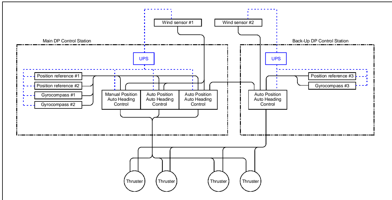
Figure DPS3: Example DPS-3 Control System Arrangement
